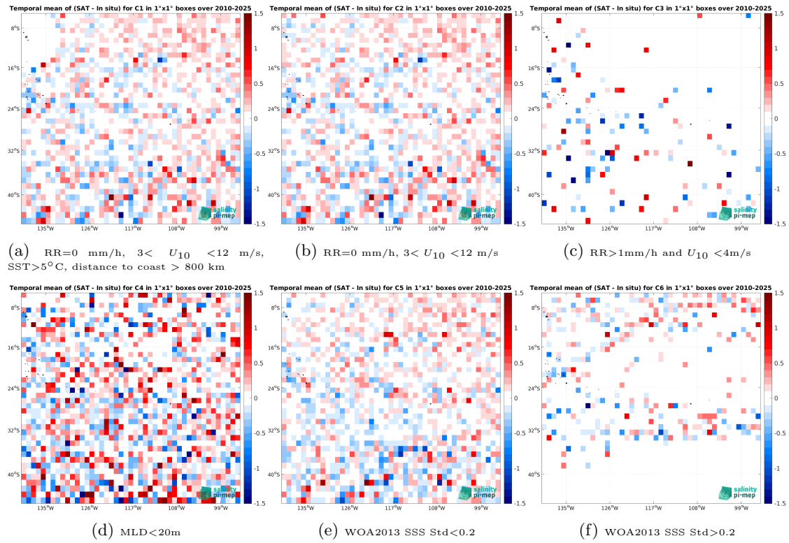
Figure 23: Temporal mean gridded over spatial boxes of size 1^\circ \times 1^\circ of \Delta SSS (SMOS SSS L2 v700 (ESA) - Argo) for 6 different subdatasets corresponding to: RR=0 mm/h, 3 < U_{10} < 12 m/s, SST > 5^\circ C , distance to coast > 800 km (a), RR=0 mm/h, 3 < U_{10} < 12 m/s (b), RR > 1 mm/h and U_{10} < 4 m/s (c), MLD < 20 m (d), WOA2013 SSS Std < 0.2 (e), WOA2013 SSS Std > 0.2 (f).
