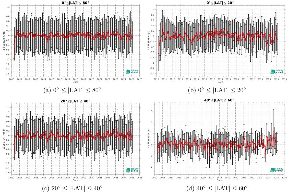
Figure 21: Monthly median (red curves) of \Delta SSS (Satellite - Argo) and \pm 1 Std (black vertical thick bars) as function of time for all the collected Pi-MEP match-up pairs estimated over the OTT zone Pi-MEP region and for the full satellite product period are shown for different latitude bands: (a) 80^\circ S-80^\circ N , (b) 20^\circ S-20^\circ N , (c) 40^\circ S-20^\circ S and 20^\circ N-40^\circ N and (d) 60^\circ S-40^\circ S and 40^\circ N-60^\circ N .
