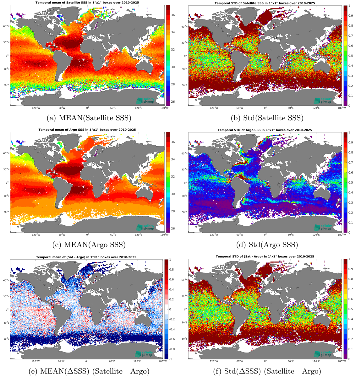
Figure 8: Temporal mean (left) and Std (right) of SSS from SMOS SSS L2 v700 (ESA) (top), Argo (middle), and of \Delta\text{SSS} (Satellite - Argo). Only match-up pairs and ascending orbits are used to generate these maps.
