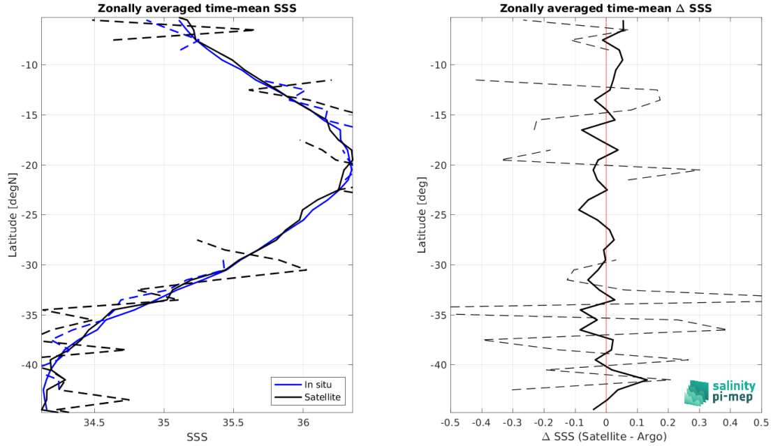
Figure 15: Left panel: Zonal mean SSS from SMOS SSS L2 v700 (ESA) satellite product (black) and from Argo (blue). Right panel: Zonal mean of \Delta\text{SSS} (Satellite - Argo) considering only descending orbits from all the collected Pi-MEP match-up pairs estimated over the full satellite product period. The dash curves correspond to the same estimates but considering only the last month of data.
