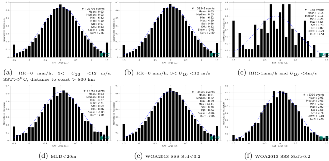
Figure 24: Normalized histogram of \Delta SSS (SMOS SSS L2 v700 (ESA) - Argo) for 6 different subdatasets corresponding to: RR=0 mm/h, 3 < U_{10} < 12 m/s, SST > 5°C, distance to coast > 800 km (a), RR=0 mm/h, 3 < U_{10} < 12 m/s (b), RR > 1mm/h and U_{10} < 4 m/s (c), MLD < 20m (d), WOA2013 SSS Std < 0.2 (e), WOA2013 SSS Std > 0.2 (f).
