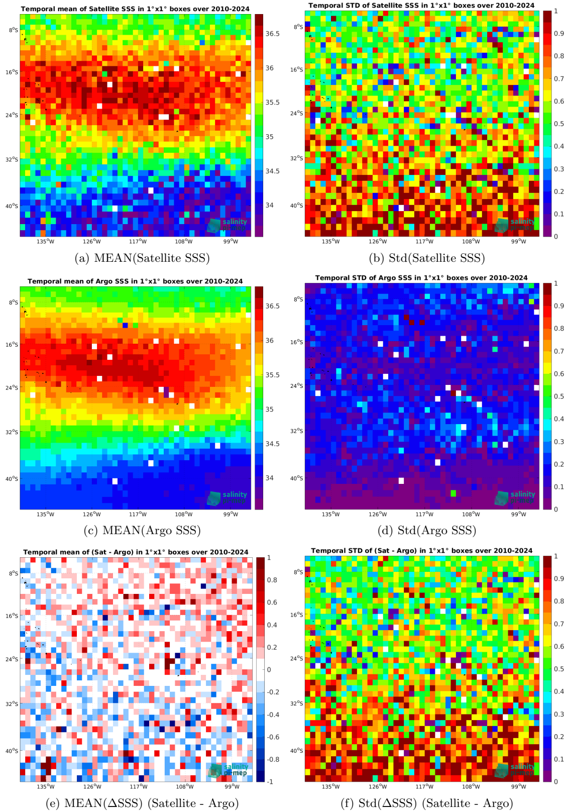
Figure 8: Temporal mean (left) and Std (right) of SSS from SMOS SSS L2 v700 (ESA) (top), Argo (middle), and of \Delta\text{SSS} (Satellite - Argo). Only match-up pairs and ascending orbits are used to generate these maps.
