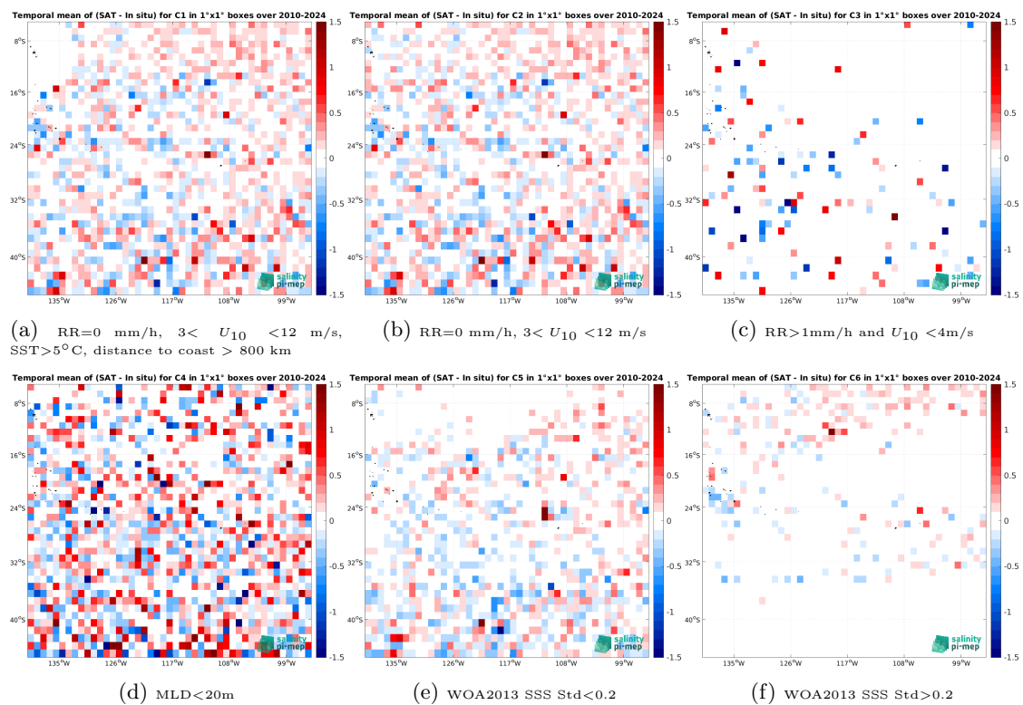
Figure 23: Temporal mean gridded over spatial boxes of size 1^\circ \times 1^\circ of \Delta SSS (SMOS SSS L2 v700 (ESA) - Argo) for 6 different subdatasets corresponding to:RR=0 mm/h, 3 < U_{10} < 12 m/s, SST >5^\circ C, distance to coast > 800 km (a), RR=0 mm/h, 3 < U_{10} < 12 m/s (b), RR >1 mm/h and U_{10} < 4 m/s (c),MLD <20 m (d),WOA2013 SSS Std <0.2 (e),WOA2013 SSS Std >0.2 (f).
