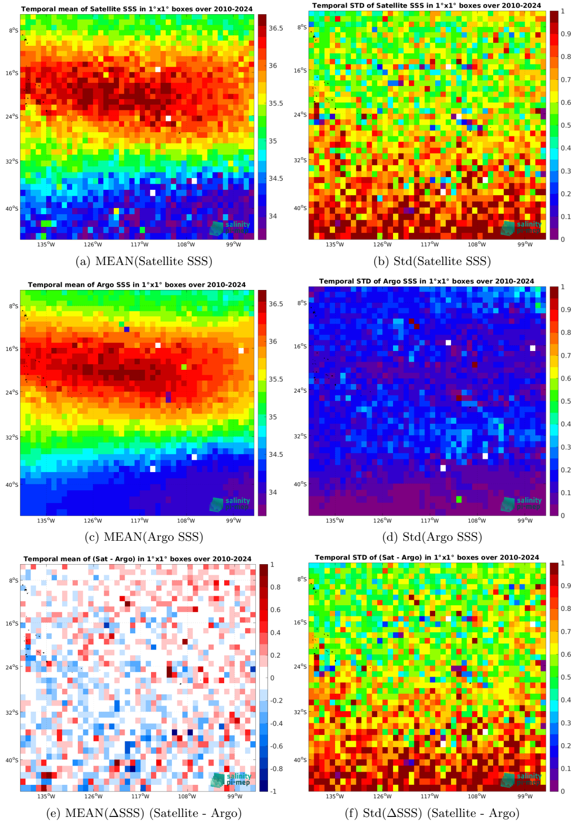
Figure 7: Temporal mean (left) and Std (right) of SSS from SMOS SSS L2 v700 (ESA) (top), Argo (middle), and of \Delta\text{SSS} (Satellite - Argo). Only match-up pairs are used to generate these maps.
