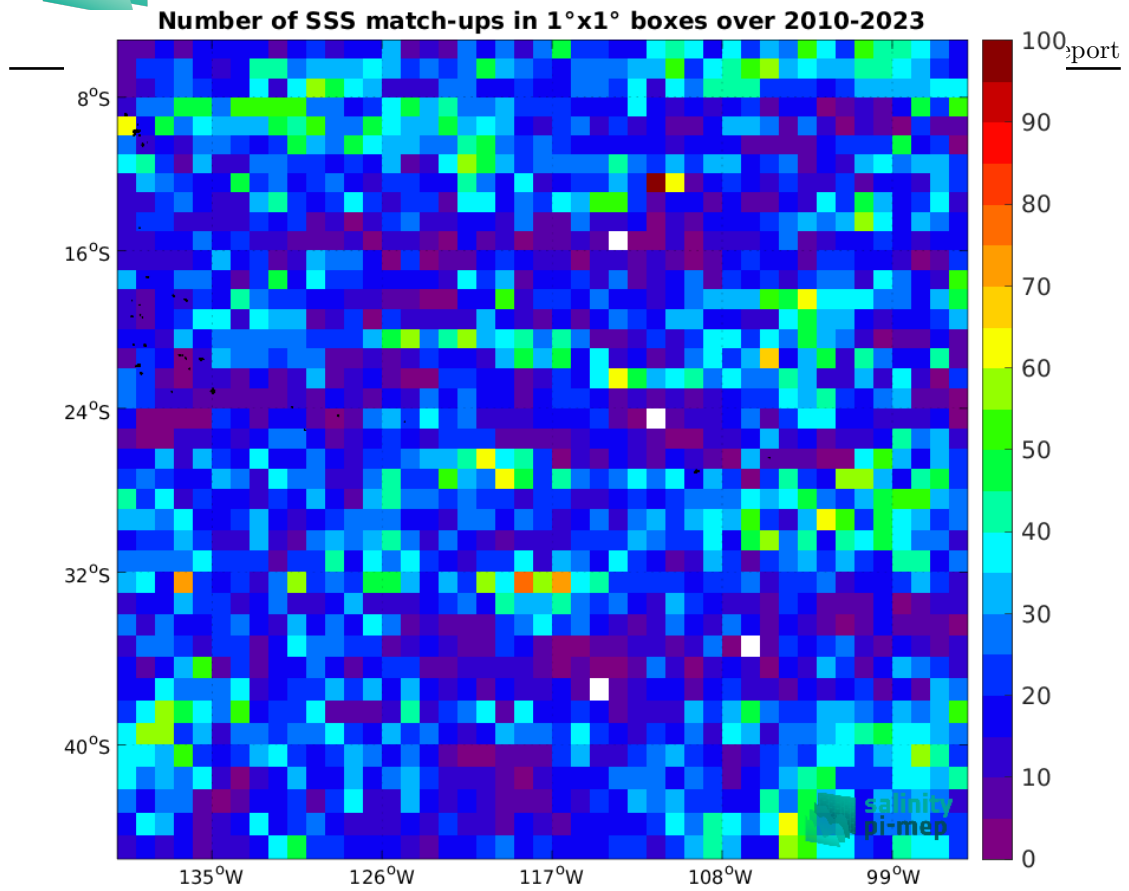
Figure 4: Number of SSS match-ups between Argo SSS and the SMOS SSS L2 v700 (ESA) SSS product for the OTT zone Pi-MEP region over 1°x1° boxes and for the full satellite product period.
