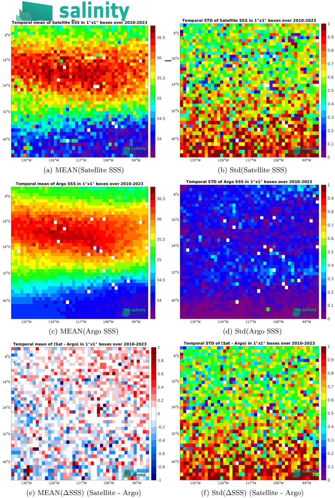
Figure 7: Temporal mean (left) and Std (right) of SSS from SMOS SSS L2 v700 (ESA) (top), Argo (middle), and of \Delta SSS (Satellite - Argo). Only match-up pairs and ascending orbits are used to generate these maps.
