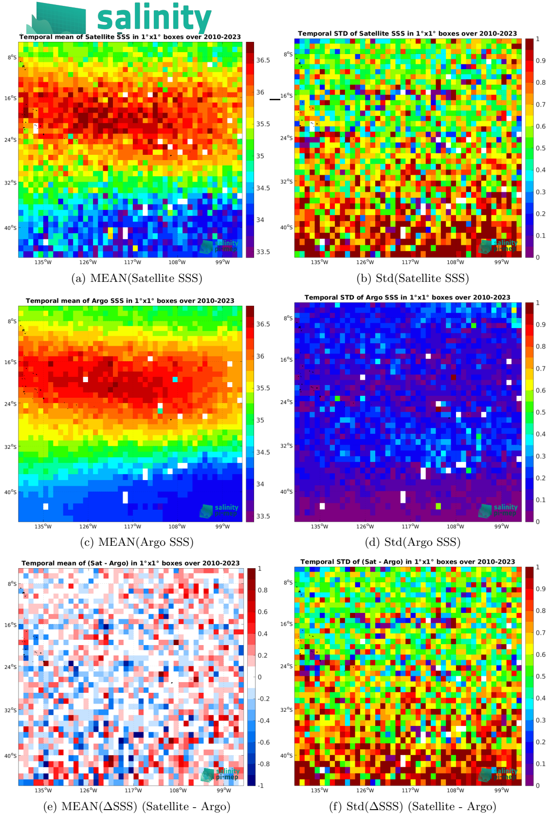
Figure 8: Temporal mean (left) and Std (right) of SSS from SMOS SSS L2 v700 (ESA) (top), Argo (middle), and of \Delta SSS (Satellite - Argo). Only match-up pairs and descending orbits are used to generate these maps.
