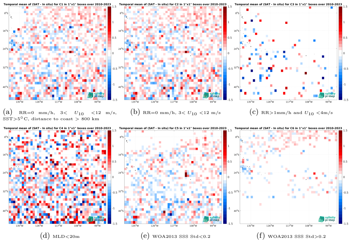
Figure 22: Temporal mean gridded over spatial boxes of size 1^\circ \times 1^\circ of \Delta SSS (SMOS SSS L2 v700 (ESA) - Argo) for 6 different subdatasets corresponding to:RR=0 mm/h, 3 < U_{10} < 12 m/s, SST >5^\circ C, distance to coast > 800 km (a), RR=0 mm/h, 3 < U_{10} < 12 m/s (b), RR >1 mm/h and U_{10} < 4 m/s (c),MLD <20 m (d),WOA2013 SSS Std <0.2 (e),WOA2013 SSS Std >0.2 (f).
