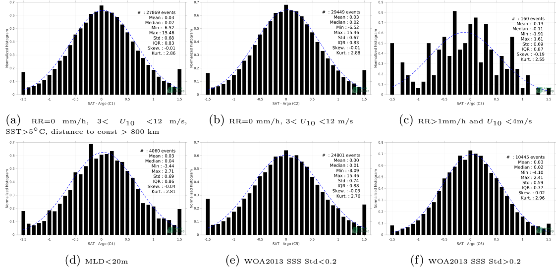
Figure 23: Normalized histogram of \Delta SSS (SMOS SSS L2 v700 (ESA) - Argo) for 6 different subdatasets corresponding to: RR=0 mm/h, 3 < U_{10} < 12 m/s, SST > 5°C, distance to coast > 800 km (a), RR=0 mm/h, 3 < U_{10} < 12 m/s (b), RR > 1mm/h and U_{10} < 4 m/s (c), MLD < 20m (d), WOA2013 SSS Std < 0.2 (e), WOA2013 SSS Std > 0.2 (f).
