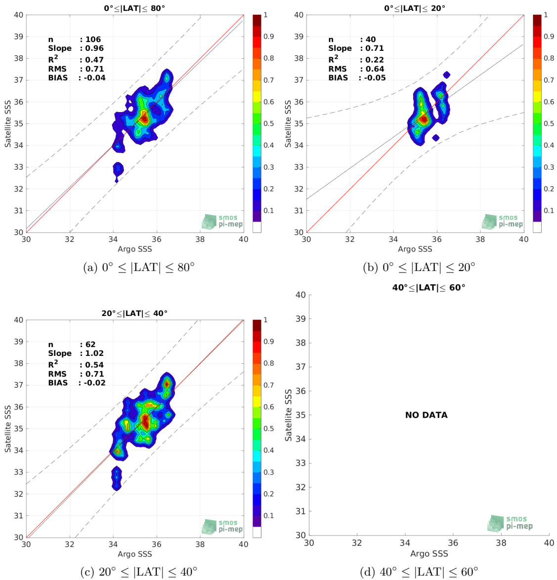
Figure 17: Contour maps of the concentration of SMOS SSS L2 v700 (ESA) SSS (y-axis) versus Argo SSS (x-axis) at match-up pairs for different latitude bands. For each plot, the red line shows x=y . The black thin and dashed lines indicate a linear fit through the data cloud and the \pm 95\% confidence levels, respectively. The number match-up pairs n , the slope and R^2 coefficient of the linear fit, the root mean square (RMS) and the mean bias between satellite and in situ data are indicated for each latitude band in each plots.
