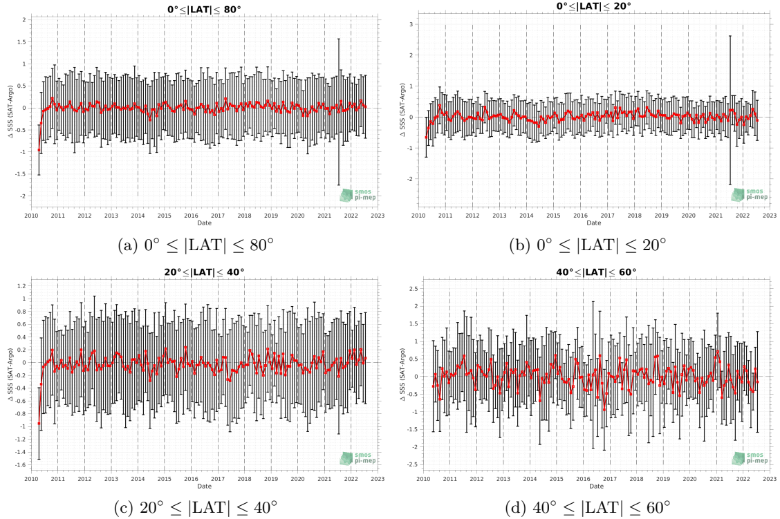
Figure 20: Monthly median (red curves) of \Delta SSS (Satellite - Argo) and \pm 1 Std (black vertical thick bars) as function of time for all the collected Pi-MEP match-up pairs estimated over the OTT zone Pi-MEP region and for the full satellite product period are shown for different latitude bands: (a) 80^\circ S-80^\circ N , (b) 20^\circ S-20^\circ N , (c) 40^\circ S-20^\circ S and 20^\circ N-40^\circ N and (d) 60^\circ S-40^\circ S and 40^\circ N-60^\circ N .
