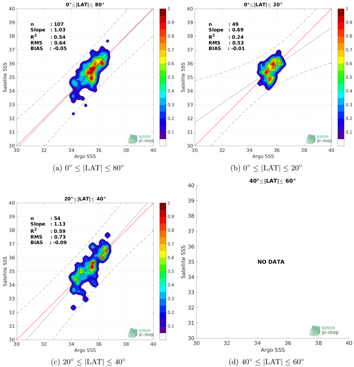
Figure 16: Contour maps of the concentration of SMOS SSS L2 v700 (ESA) SSS (y-axis) versus Argo SSS (x-axis) at match-up pairs for different latitude bands. For each plot, the red line shows x=y . The black thin and dashed lines indicate a linear fit through the data cloud and the \pm 95\% confidence levels, respectively. The number match-up pairs n , the slope and R^2 coefficient of the linear fit, the root mean square (RMS) and the mean bias between satellite and in situ data are indicated for each latitude band in each plots.
