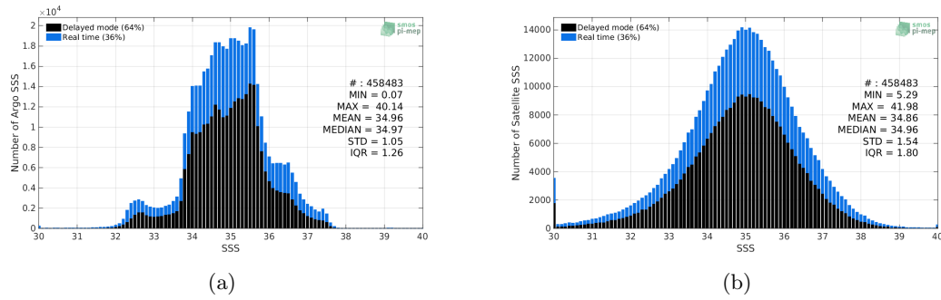
Figure 2: Histograms of SSS from Argo (a) and SMOS-L2-DPGS-v662 (b) considering all match-up pairs per bins of 0.1 over the Global Ocean Pi-MEP region and for the full satellite product period.
