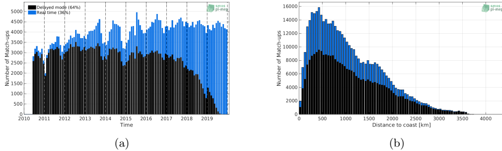
Figure 1: Number of match-ups between Argo and SMOS-L2-DPGS-v662 SSS as a function of time (a) and as function of the distance to coast (b) over the Global Ocean Pi-MEP region and for the full satellite product period.
