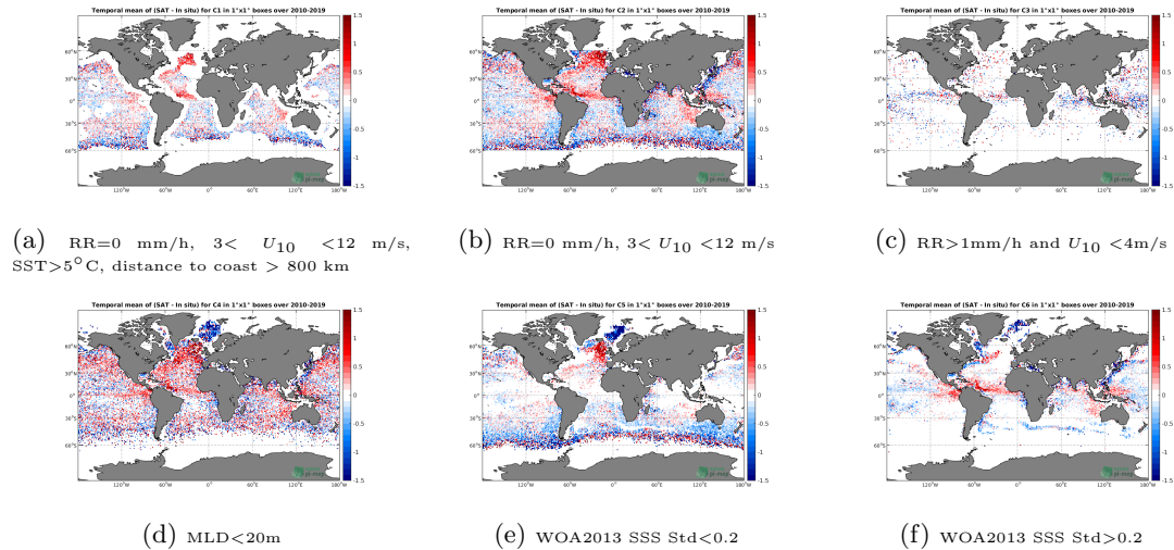
Figure 12: Temporal mean gridded over spatial boxes of size 1^\circ \times 1^\circ of \Delta\text{SSS} (SMOS-L2-DPGS-v662 - Argo) for 6 different subdatasets corresponding to: \text{RR}=0 \text{ mm/h} , 3 < U_{10} < 12 \text{ m/s} , \text{SST} > 5^\circ\text{C} , distance to coast > 800 \text{ km} (a), \text{RR}=0 \text{ mm/h} , 3 < U_{10} < 12 \text{ m/s} (b), \text{RR} > 1 \text{ mm/h} and U_{10} < 4 \text{ m/s} (c), \text{MLD} < 20 \text{ m} (d), \text{WOA2013 SSS Std} < 0.2 (e), \text{WOA2013 SSS Std} > 0.2 (f).
