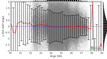
(a) Argo SSS
