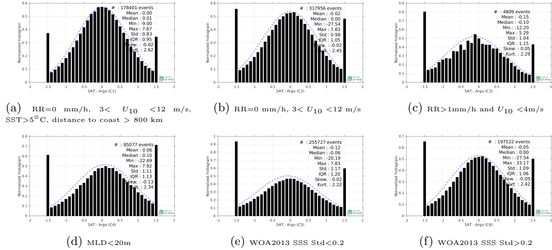
Figure 13: Normalized histogram of \Delta SSS (SMOS-L2-DPGS-v662 - Argo) for 6 different sub-datasets corresponding to: RR=0 mm/h, 3 < U_{10} < 12 m/s, SST>5°C, distance to coast > 800 km (a), RR=0 mm/h, 3 < U_{10} < 12 m/s (b), RR>1mm/h and U_{10} < 4 m/s (c), MLD<20m (d), WOA2013 SSS Std<0.2 (e), WOA2013 SSS Std>0.2 (f).
