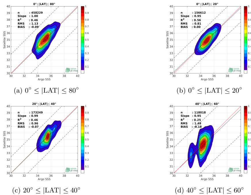
Figure 9: Contour maps of the concentration of SMOS-L2-DPGS-v662 SSS (y-axis) versus Argo SSS (x-axis) at match-up pairs for different latitude bands. For each plot, the red line shows x=y . The black thin and dashed lines indicate a linear fit through the data cloud and the \pm 95\% confidence levels, respectively. The number match-up pairs n , the slope and R^2 coefficient of the linear fit, the root mean square (RMS) and the mean bias between satellite and in situ data are indicated for each latitude band in each plots.
