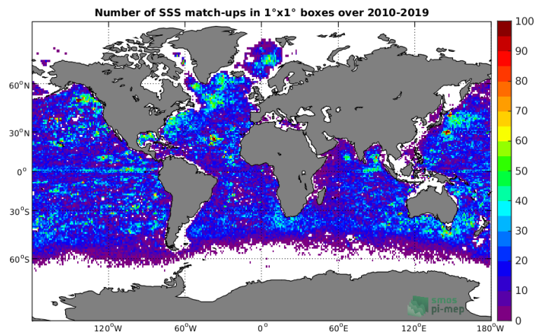
Figure 4: Number of SSS match-ups between Argo SSS and the SMOS-L2-DPGS-v662 SSS product for the Global Ocean Pi-MEP region over 1^\circ \times 1^\circ boxes and for the full satellite product period.
