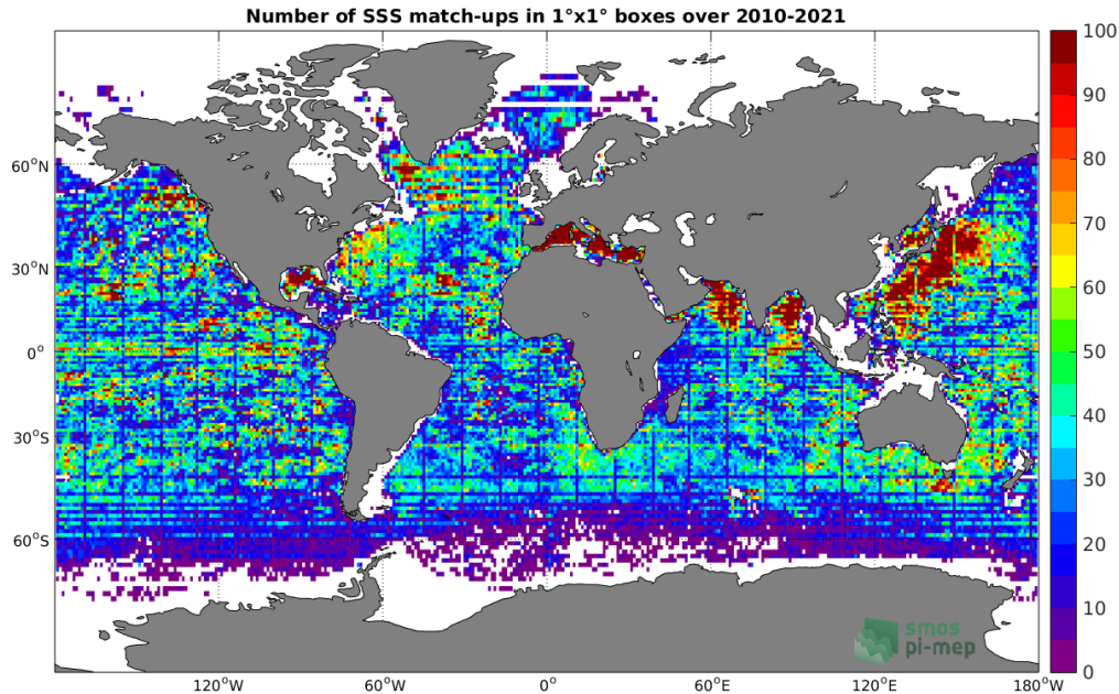
Figure 4: Number of SSS match-ups between Argo SSS and the SMOS SSS L3 v335 - Monthly - 50 km (CATDS-CPDC) SSS product for the Global Ocean Pi-MEP region over 1^\circ \times 1^\circ boxes and for the full satellite product period.
