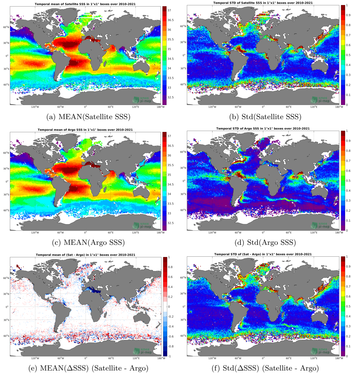
Figure 6: Temporal mean (left) and Std (right) of SSS from SMOS SSS L3 v335 - Monthly - 50 km (CATDS-CPDC) (top), Argo (middle), and of \Delta SSS (Satellite - Argo). Only match-up pairs are used to generate these maps.
