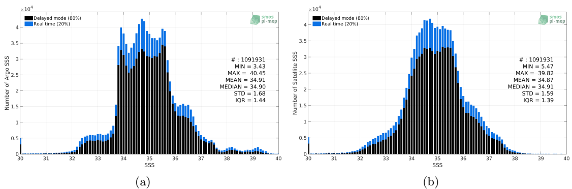
Figure 2: Histograms of SSS from Argo (a) and SMOS SSS L3 v335 - Monthly - 50 km (CATDS-CPDC) (b) considering all match-up pairs per bins of 0.1 over the Global Ocean Pi-MEP region and for the full satellite product period.
