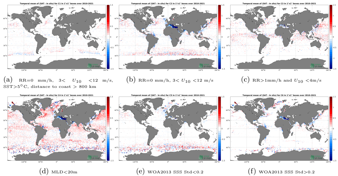
Figure 12: Temporal mean gridded over spatial boxes of size 1^\circ \times 1^\circ of \Delta SSS (SMOS SSS L3 v335 - Monthly - 50 km (CATDS-CPDC) - Argo) for 6 different subdatasets corresponding to:RR=0 mm/h, 3 < U_{10} < 12 m/s, SST > 5°C, distance to coast > 800 km (a), RR=0 mm/h, 3 < U_{10} < 12 m/s (b), RR > 1mm/h and U_{10} < 4 m/s (c),MLD < 20m (d),WOA2013 SSS Std < 0.2 (e),WOA2013 SSS Std > 0.2 (f).
