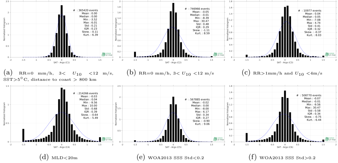
Figure 13: Normalized histogram of \Delta SSS (SMOS SSS L3 v335 - Monthly - 50 km (CATDS-CPDC) - Argo) for 6 different subdatasets corresponding to: RR=0 mm/h, 3 < U_{10} < 12 m/s, SST>5°C, distance to coast > 800 km (a), RR=0 mm/h, 3 < U_{10} < 12 m/s (b), RR>1mm/h and U_{10} < 4 m/s (c), MLD<20m (d), WOA2013 SSS Std<0.2 (e), WOA2013 SSS Std>0.2 (f).
