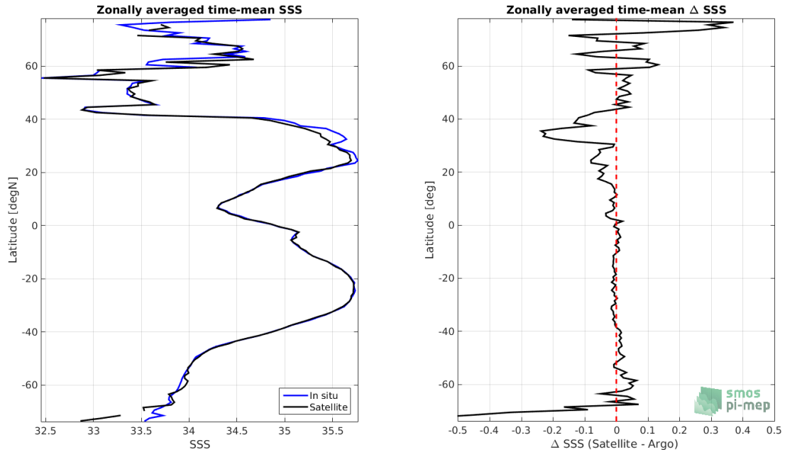
Figure 8: Left panel: Zonal mean SSS from SMOS SSS L3 v335 - Monthly - 50 km (CATDS-CPDC) satellite product (black) and from Argo (blue). Right panel: Zonal mean of \Delta SSS (Satellite - Argo) for all the collected Pi-MEP match-up pairs estimated over the full satellite product period.
