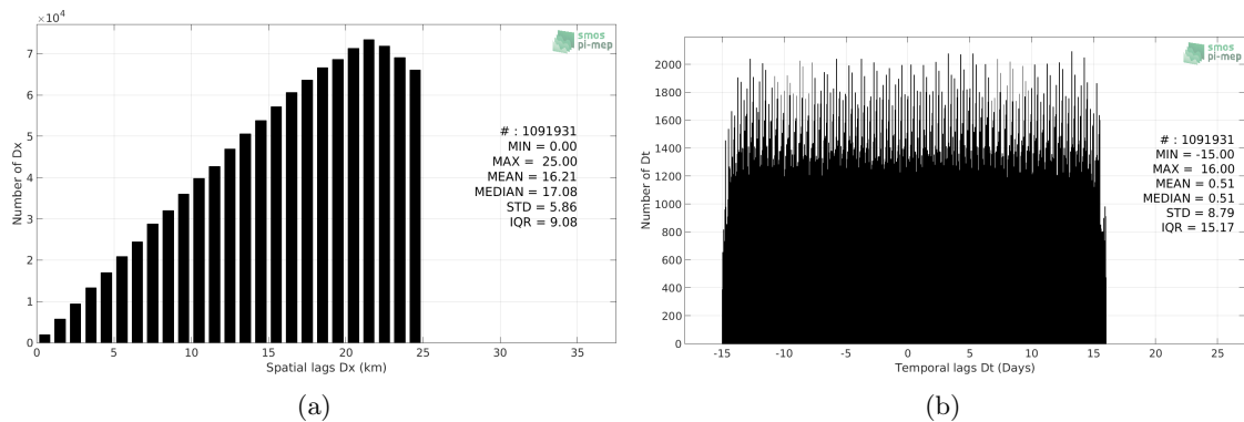
Figure 5: Histograms of the spatial (a) and temporal (b) lags between the location/time of the Argo measurement and the date of the corresponding SMOS SSS L3 v335 - Monthly - 50 km (CATDS-CPDC) SSS pixel.
