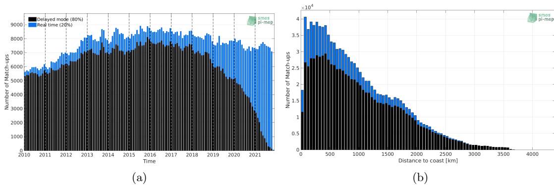
Figure 1: Number of match-ups between Argo and SMOS SSS L3 v335 - Monthly - 50 km (CATDS-CPDC) SSS as a function of time (a) and as function of the distance to coast (b) over the Global Ocean Pi-MEP region and for the full satellite product period.
