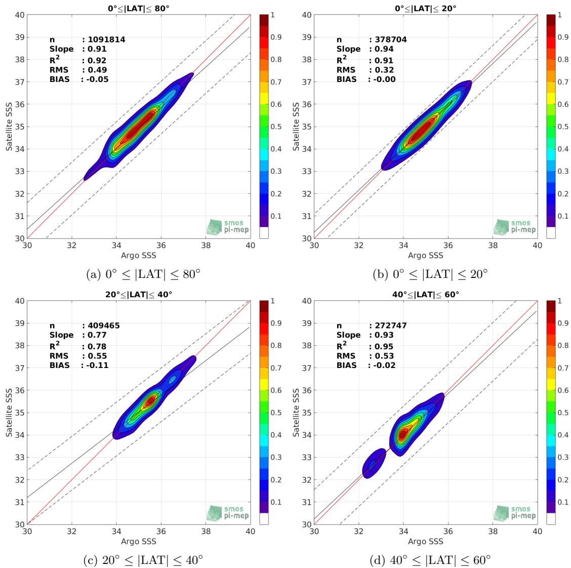
Figure 9: Contour maps of the concentration of SMOS SSS L3 v335 - Monthly - 50 km (CATDS-CPDC) SSS (y-axis) versus Argo SSS (x-axis) at match-up pairs for different latitude bands. For each plot, the red line shows x=y . The black thin and dashed lines indicate a linear fit through the data cloud and the \pm 95\% confidence levels, respectively. The number match-up pairs n , the slope and R^2 coefficient of the linear fit, the root mean square (RMS) and the mean bias between satellite and in situ data are indicated for each latitude band in each plots.
