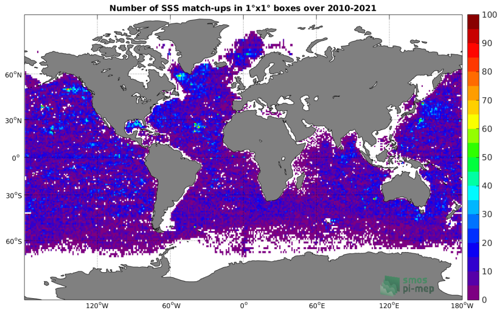
Figure 4: Number of SSS match-ups between Argo SSS and the SMOS SSS L2Q v330 - Ascending - 0.25 Deg (CATDS-CPDC) SSS product for the Global Ocean Pi-MEP region over 1^\circ \times 1^\circ boxes and for the full satellite product period.
