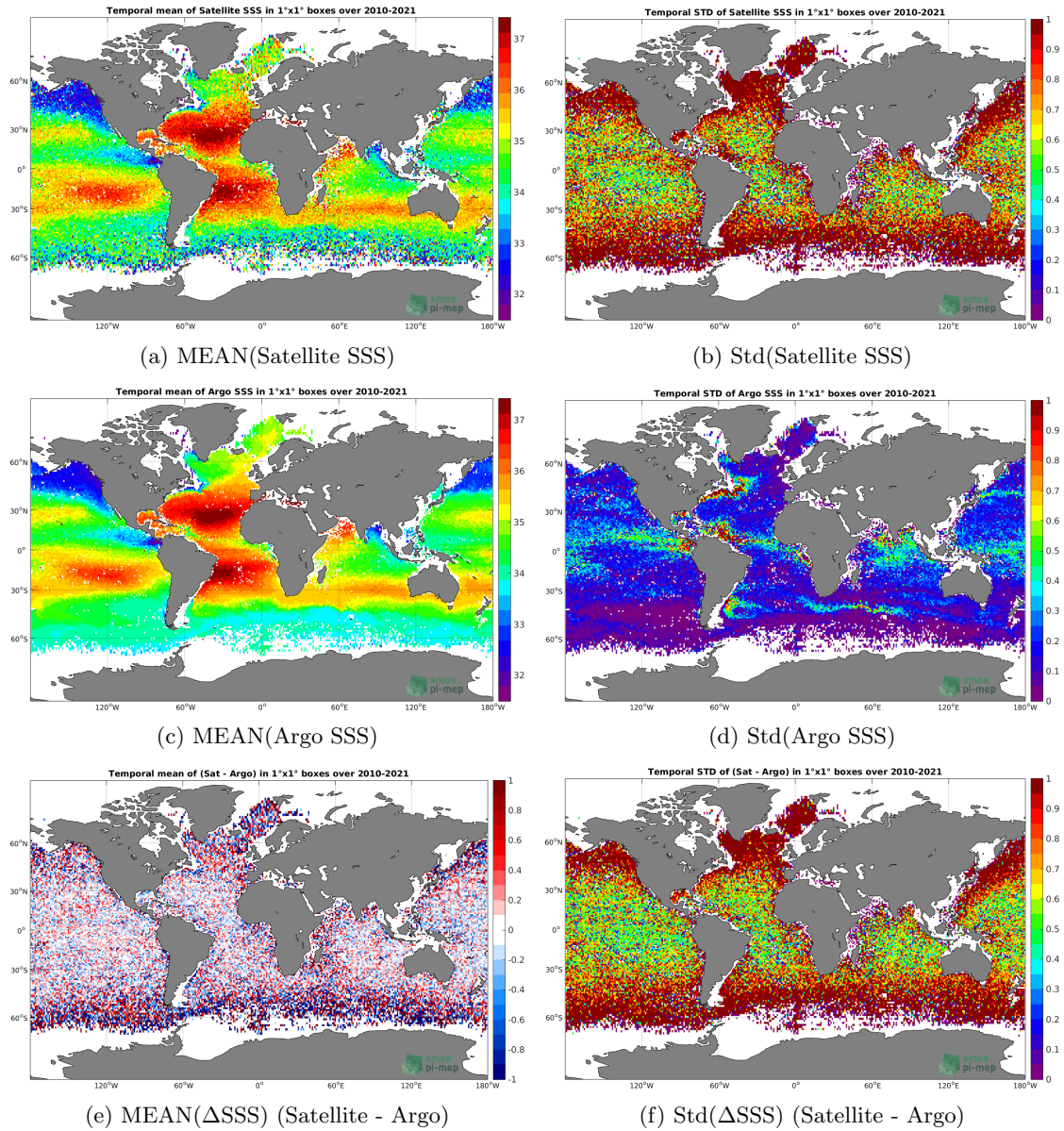
Figure 6: Temporal mean (left) and Std (right) of SSS from SMOS SSS L2Q v330 - Ascending - 0.25 Deg (CATDS-CPDC) (top), Argo (middle), and of \Delta SSS (Satellite - Argo). Only match-up pairs are used to generate these maps.
