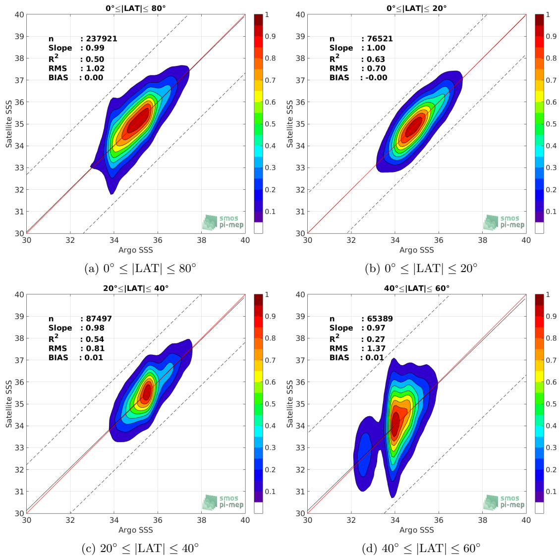
Figure 9: Contour maps of the concentration of SMOS SSS L2Q v330 - Ascending - 0.25 Deg (CATDS-CPDC) SSS (y-axis) versus Argo SSS (x-axis) at match-up pairs for different latitude bands. For each plot, the red line shows x=y . The black thin and dashed lines indicate a linear fit through the data cloud and the \pm 95\% confidence levels, respectively. The number match-up pairs n , the slope and R^2 coefficient of the linear fit, the root mean square (RMS) and the mean bias between satellite and in situ data are indicated for each latitude band in each plots.
