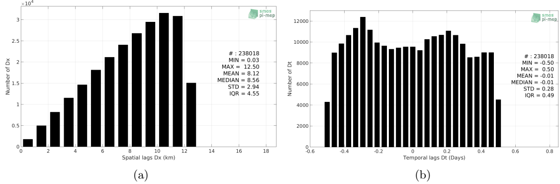
Figure 5: Histograms of the spatial (a) and temporal (b) lags between the location/time of the Argo measurement and the date of the corresponding SMOS SSS L2Q v330 - Ascending - 0.25 Deg (CATDS-CPDC) SSS pixel.
