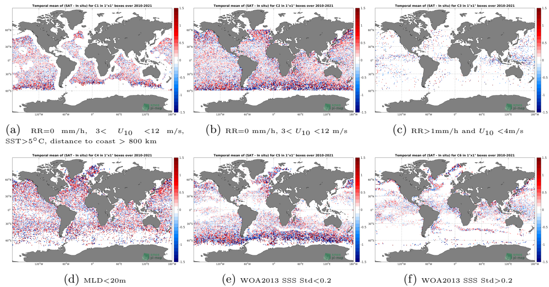
Figure 12: Temporal mean gridded over spatial boxes of size 1^\circ \times 1^\circ of \Delta SSS (SMOS SSS L2Q v330 - Ascending - 0.25 Deg (CATDS-CPDC) - Argo) for 6 different subdatasets corresponding to:RR=0 mm/h, 3 < U_{10} < 12 m/s, SST > 5^\circ\text{C} , distance to coast > 800 km (a), RR=0 mm/h, 3 < U_{10} < 12 m/s (b), RR > 1 mm/h and U_{10} < 4 m/s (c),MLD < 20 m (d),WOA2013 SSS Std < 0.2 (e),WOA2013 SSS Std > 0.2 (f).
