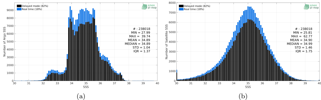
Figure 2: Histograms of SSS from Argo (a) and SMOS SSS L2Q v330 - Ascending - 0.25 Deg (CATDS-CPDC) (b) considering all match-up pairs per bins of 0.1 over the Global Ocean Pi-MEP region and for the full satellite product period.
