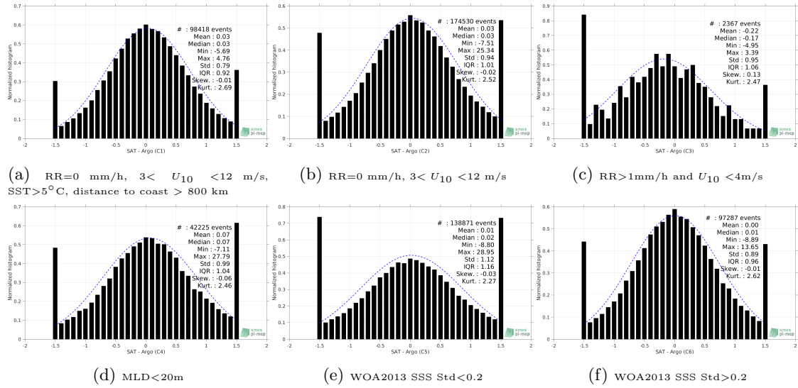
Figure 13: Normalized histogram of \Delta SSS (SMOS SSS L2Q v330 - Ascending - 0.25 Deg (CATDS-CPDC) - Argo) for 6 different subdatasets corresponding to: RR=0 mm/h, 3 < U_{10} < 12 m/s, SST>5°C, distance to coast > 800 km (a), RR=0 mm/h, 3 < U_{10} < 12 m/s (b), RR>1mm/h and U_{10} < 4 m/s (c), MLD<20m (d), WOA2013 SSS Std<0.2 (e), WOA2013 SSS Std>0.2 (f).
