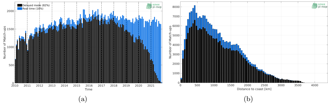
Figure 1: Number of match-ups between Argo and SMOS SSS L2Q v330 - Ascending - 0.25 Deg (CATDS-CPDC) SSS as a function of time (a) and as function of the distance to coast (b) over the Global Ocean Pi-MEP region and for the full satellite product period.
