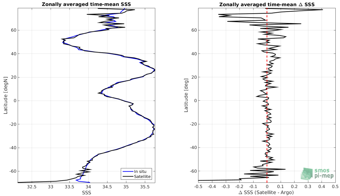
Figure 8: Left panel: Zonal mean SSS from SMOS SSS L2Q v330 - Ascending - 0.25 Deg (CATDS-CPDC) satellite product (black) and from Argo (blue). Right panel: Zonal mean of \Delta SSS (Satellite - Argo) for all the collected Pi-MEP match-up pairs estimated over the full satellite product period.
