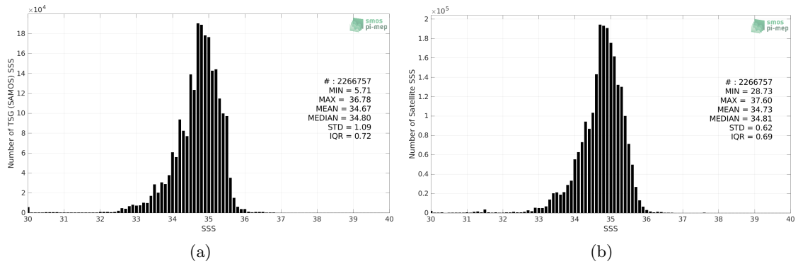
Figure 2: Histograms of SSS from TSG (SAMOS) (a) and SMOS and SMAP SSS L4 OI v1 - 7 Days (LOPS) (b) considering all match-up pairs per bins of 0.1 over the Tropical Pacific Ocean Pi-MEP region and for the full satellite product period.
