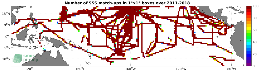
Figure 4: Number of SSS match-ups between TSG (SAMOS) SSS and the SMOS and SMAP SSS L4 OI v1 - 7 Days (LOPS) SSS product for the Tropical Pacific Ocean Pi-MEP region over 1^\circ \times 1^\circ boxes and for the full satellite product period.
