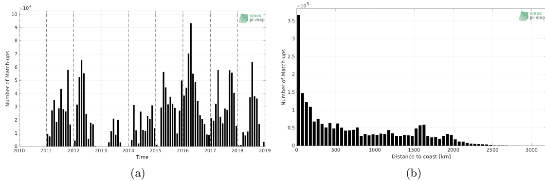
Figure 1: Number of match-ups between TSG (SAMOS) and SMOS and SMAP SSS L4 OI v1 - 7 Days (LOPS) SSS as a function of time (a) and as function of the distance to coast (b) over the Tropical Pacific Ocean Pi-MEP region and for the full satellite product period.
