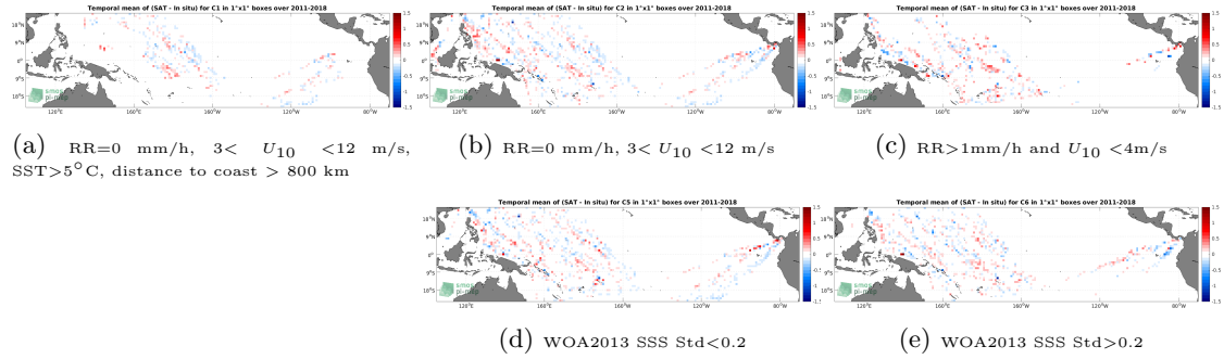
Figure 12: Temporal mean gridded over spatial boxes of size 1^{\circ}\times 1^{\circ} of \Delta\text{SSS} (SMOS and SMAP SSS L4 OI v1 - 7 Days (LOPS) - TSG (LEGOS-DM)) for 5 different subdatasets corresponding to:RR=0 mm/h, 3 < U_{10} < 12 m/s, SST > 5^{\circ}\text{C} , distance to coast > 800 km (a), RR=0 mm/h, 3 < U_{10} < 12 m/s (b), RR > 1 mm/h and U_{10} < 4 m/s (c), WOA2013 SSS Std < 0.2 (d), WOA2013 SSS Std > 0.2 (e).
