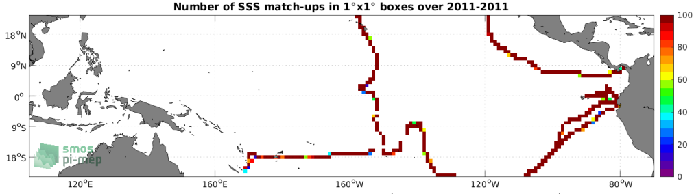
Figure 4: Number of SSS match-ups between TSG (GOSUD-Sailing-ship) SSS and the SMOS and SMAP SSS L4 OI v1 - 7 Days (LOPS) SSS product for the Tropical Pacific Ocean Pi-MEP region over 1^\circ \times 1^\circ boxes and for the full satellite product period.
