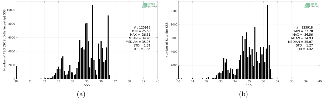
Figure 2: Histograms of SSS from TSG (GOSUD-Sailing-ship) (a) and SMOS and SMAP SSS L4 OI v1 - 7 Days (LOPS) (b) considering all match-up pairs per bins of 0.1 over the Tropical Pacific Ocean Pi-MEP region and for the full satellite product period.
