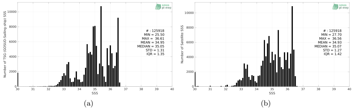
Figure 2: Histograms of SSS from TSG (GOSUD-Sailing-ship) (a) and SMOS and SMAP SSS L4 OI v1 - 7 Days (LOPS) (b) considering all match-up pairs per bins of 0.1 over the Tropical Pacific Ocean Pi-MEP region and for the full satellite product period.
