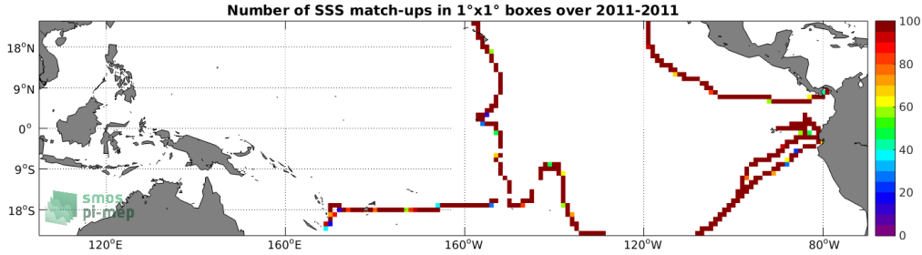
Figure 4: Number of SSS match-ups between TSG (GOSUD-Sailing-ship) SSS and the SMOS and SMAP SSS L4 OI v1 - 7 Days (LOPS) SSS product for the Tropical Pacific Ocean Pi-MEP region over 1^\circ \times 1^\circ boxes and for the full satellite product period.
