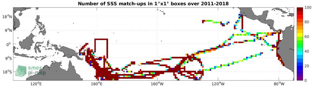
Figure 4: Number of SSS match-ups between TSG (GOSUD-Research-vessel) SSS and the SMOS and SMAP SSS L4 OI v1 - 7 Days (LOPS) SSS product for the Tropical Pacific Ocean Pi-MEP region over 1^\circ \times 1^\circ boxes and for the full satellite product period.
