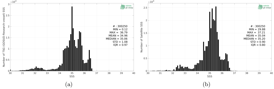
Figure 2: Histograms of SSS from TSG (GOSUD-Research-vessel) (a) and SMOS and SMAP SSS L4 OI v1 - 7 Days (LOPS) (b) considering all match-up pairs per bins of 0.1 over the Tropical Pacific Ocean Pi-MEP region and for the full satellite product period.
