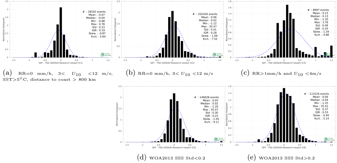
Figure 13: Normalized histogram of \Delta\text{SSS} (SMOS and SMAP SSS L4 OI v1 - 7 Days (LOPS) - TSG (GOSUD-Research-vessel)) for 5 different subdatasets corresponding to: RR=0 mm/h, 3 < U_{10} < 12 m/s, SST>5°C, distance to coast > 800 km (a), RR=0 mm/h, 3 < U_{10} < 12 m/s (b), RR>1mm/h and U_{10} < 4 m/s (c), WOA2013 SSS Std<0.2 (d), WOA2013 SSS Std>0.2 (e).
