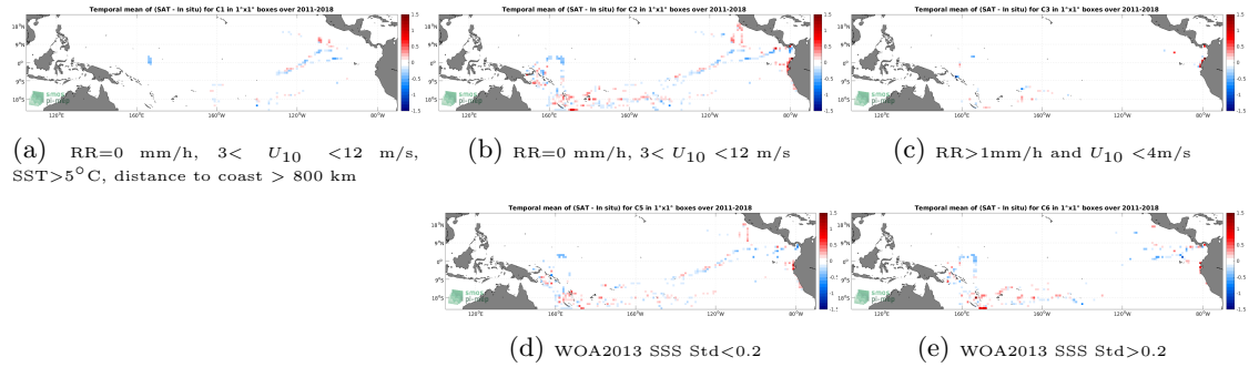
Figure 12: Temporal mean gridded over spatial boxes of size 1^{\circ}\times 1^{\circ} of \Delta SSS (SMOS and SMAP SSS L4 OI v1 - 7 Days (LOPS) - TSG (GOSUD-Research-vessel)) for 5 different subdatasets corresponding to:RR=0 mm/h, 3 < U_{10} < 12 m/s, SST >5^{\circ}\text{C} , distance to coast > 800 km (a), RR=0 mm/h, 3 < U_{10} < 12 m/s (b), RR >1 mm/h and U_{10} < 4 m/s (c), WOA2013 SSS Std <0.2 (d), WOA2013 SSS Std >0.2 (e).
