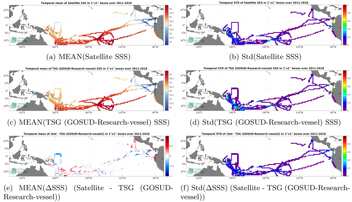
Figure 6: Temporal mean (left) and Std (right) of SSS from SMOS and SMAP SSS L4 OI v1 - 7 Days (LOPS) (top), TSG (GOSUD-Research-vessel) (middle), and of \Delta SSS (Satellite - TSG (GOSUD-Research-vessel)). Only match-up pairs are used to generate these maps.
