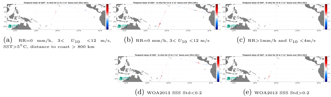
Figure 12: Temporal mean gridded over spatial boxes of size 1^\circ \times 1^\circ of \Delta SSS (SMOS and SMAP SSS L4 OI v1 - 7 Days (LOPS) - TSG (CSIC-UTM)) for 5 different subdatasets corresponding to:RR=0 mm/h, 3 < U_{10} < 12 m/s, SST >5^\circ C, distance to coast > 800 km (a), RR=0 mm/h, 3 < U_{10} < 12 m/s (b), RR >1 mm/h and U_{10} < 4 m/s (c), WOA2013 SSS Std <0.2 (d), WOA2013 SSS Std >0.2 (e).
