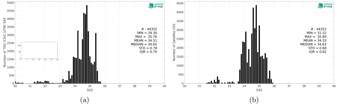
Figure 2: Histograms of SSS from TSG (CSIC-UTM) (a) and SMOS and SMAP SSS L4 OI v1 - 7 Days (LOPS) (b) considering all match-up pairs per bins of 0.1 over the Tropical Pacific Ocean Pi-MEP region and for the full satellite product period.
