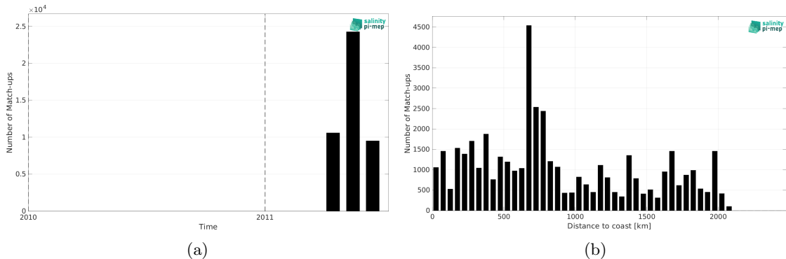
Figure 1: Number of match-ups between TSG (CSIC-UTM) and SMOS and SMAP SSS L4 OI v1 - 7 Days (LOPS) SSS as a function of time (a) and as function of the distance to coast (b) over the Tropical Pacific Ocean Pi-MEP region and for the full satellite product period.
