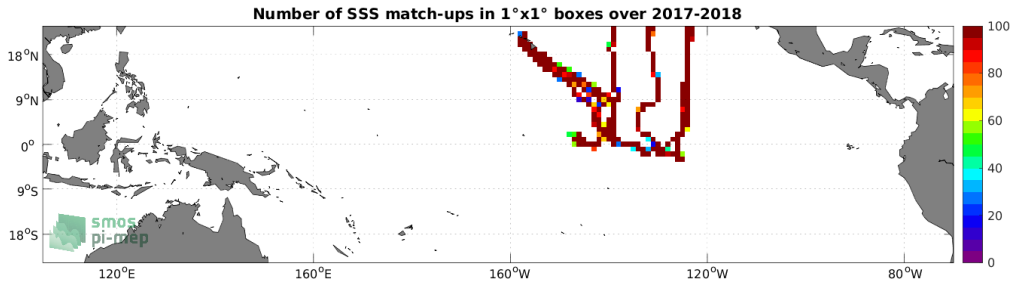
Figure 4: Number of SSS match-ups between Saildrone SSS and the SMOS and SMAP SSS L4 OI v1 - 7 Days (LOPS) SSS product for the Tropical Pacific Ocean Pi-MEP region over 1^\circ \times 1^\circ boxes and for the full satellite product period.
