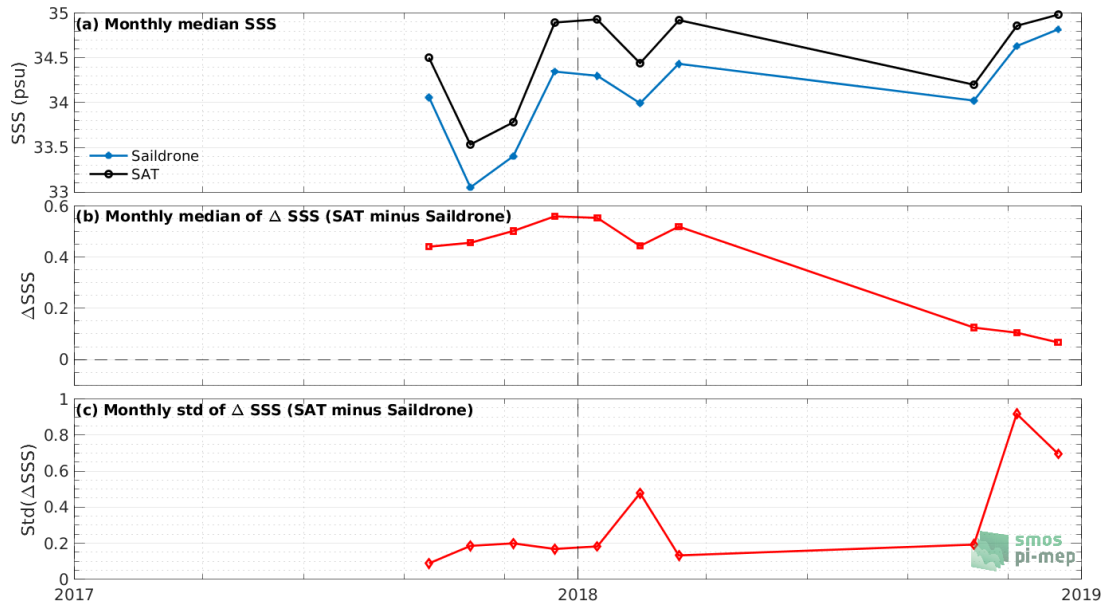
Figure 7: Time series of the monthly median SSS (top), median of \Delta SSS (Satellite - Sairdrones) and Std of \Delta SSS (Satellite - Sairdrones) over the Tropical Pacific Ocean Pi-MEP region considering all match-ups collected by the Pi-MEP.
