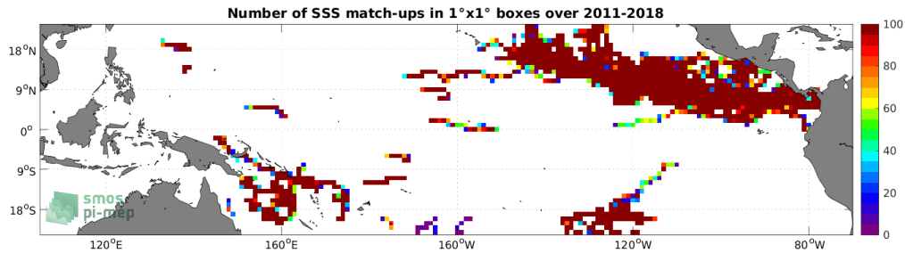
Figure 3: Number of SSS match-ups between Surface drifters SSS and the SMOS and SMAP SSS L4 OI v1 - 7 Days (LOPS) SSS product for the Tropical Pacific Ocean Pi-MEP region over 1^\circ \times 1^\circ boxes and for the full satellite product period.
