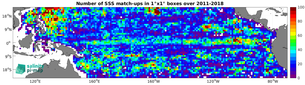
Figure 4: Number of SSS match-ups between Argo SSS and the SMOS and SMAP SSS L4 OI v1 - 7 Days (LOPS) SSS product for the Tropical Pacific Ocean Pi-MEP region over 1^\circ \times 1^\circ boxes and for the full satellite product period.
