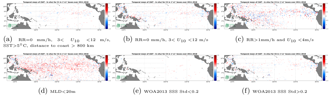
Figure 12: Temporal mean gridded over spatial boxes of size 1^\circ \times 1^\circ of \Delta SSS (SMOS and SMAP SSS L4 OI v1 - 7 Days (LOPS) - Argo) for 6 different subdatasets corresponding to: RR=0 mm/h, 3 < U_{10} < 12 m/s, SST > 5^\circ C , distance to coast > 800 km (a), RR=0 mm/h, 3 < U_{10} < 12 m/s (b), RR > 1 mm/h and U_{10} < 4 m/s (c), MLD < 20 m (d), WOA2013 SSS Std < 0.2 (e), WOA2013 SSS Std > 0.2 (f).
