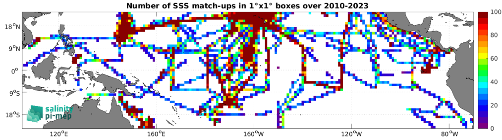
Figure 4: Number of SSS match-ups between TSG (SAMOS) SSS and the SMOS SSS L4 v1 - Weekly (CMEMS-CNR) SSS product for the Tropical Pacific Ocean Pi-MEP region over 1^\circ \times 1^\circ boxes and for the full satellite product period.
