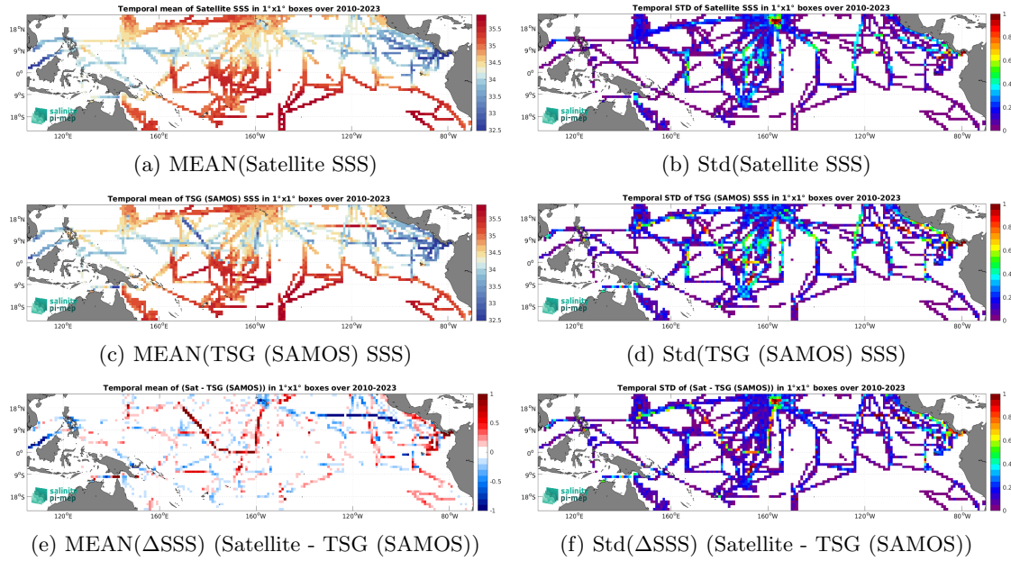
Figure 6: Temporal mean (left) and Std (right) of SSS from SMOS SSS L4 v1 - Weekly (CMEMS-CNR) (top), TSG (SAMOS) (middle), and of \Delta SSS (Satellite - TSG (SAMOS)). Only match-up pairs are used to generate these maps.
