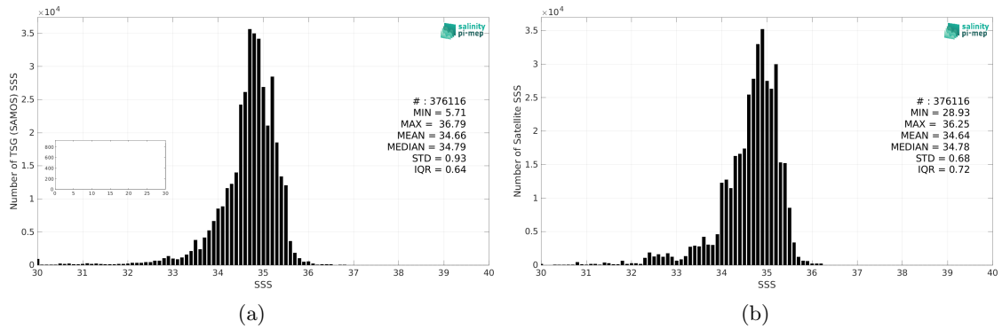
Figure 2: Histograms of SSS from TSG (SAMOS) (a) and SMOS SSS L4 v1 - Weekly (CMEMS-CNR) (b) considering all match-up pairs per bins of 0.1 over the Tropical Pacific Ocean Pi-MEP region and for the full satellite product period.
