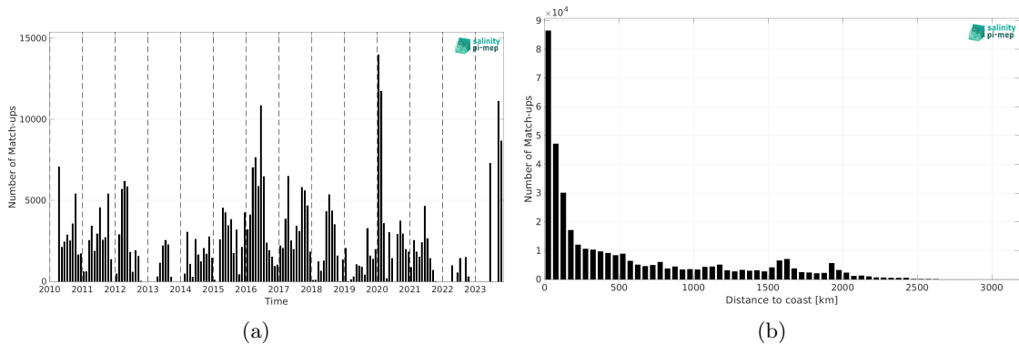
Figure 1: Number of match-ups between TSG (SAMOS) and SMOS SSS L4 v1 - Weekly (CMEMS-CNR) SSS as a function of time (a) and as function of the distance to coast (b) over the Tropical Pacific Ocean Pi-MEP region and for the full satellite product period.
