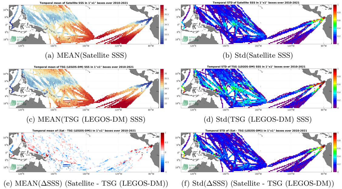
Figure 6: Temporal mean (left) and Std (right) of SSS from SMOS SSS L4 v1 - Weekly (CMEMS-CNR) (top), TSG (LEGOS-DM) (middle), and of \Delta SSS (Satellite - TSG (LEGOS-DM)). Only match-up pairs are used to generate these maps.
