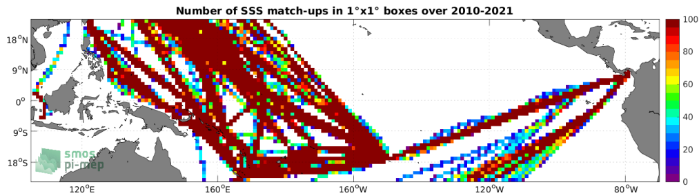
Figure 4: Number of SSS match-ups between TSG (LEGOS-DM) SSS and the SMOS SSS L4 v1 - Weekly (CMEMS-CNR) SSS product for the Tropical Pacific Ocean Pi-MEP region over 1^\circ \times 1^\circ boxes and for the full satellite product period.
