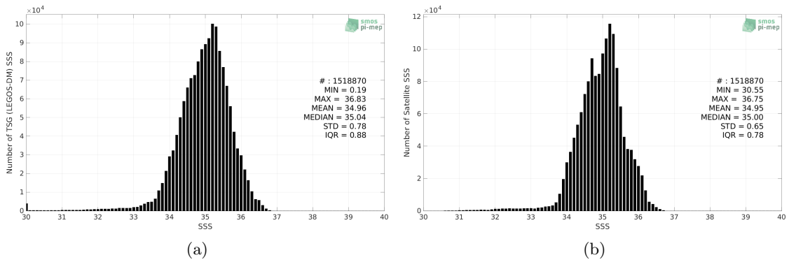
Figure 2: Histograms of SSS from TSG (LEGOS-DM) (a) and SMOS SSS L4 v1 - Weekly (CMEMS-CNR) (b) considering all match-up pairs per bins of 0.1 over the Tropical Pacific Ocean Pi-MEP region and for the full satellite product period.
