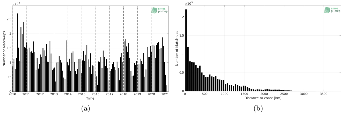
Figure 1: Number of match-ups between TSG (LEGOS-DM) and SMOS SSS L4 v1 - Weekly (CMEMS-CNR) SSS as a function of time (a) and as function of the distance to coast (b) over the Tropical Pacific Ocean Pi-MEP region and for the full satellite product period.
