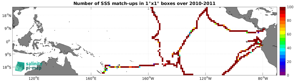
Figure 4: Number of SSS match-ups between TSG (GOSUD-Sailing-ship) SSS and the SMOS SSS L4 v1 - Weekly (CMEMS-CNR) SSS product for the Tropical Pacific Ocean Pi-MEP region over 1^\circ \times 1^\circ boxes and for the full satellite product period.
