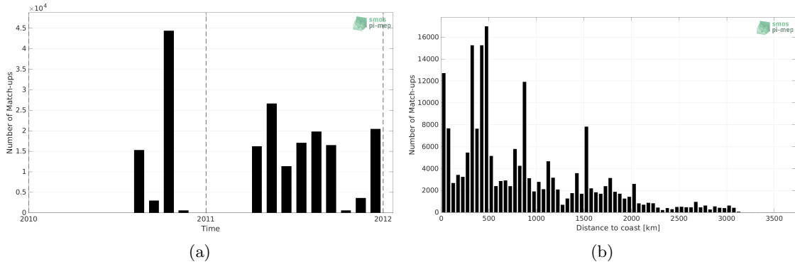
Figure 1: Number of match-ups between TSG (GOSUD-Sailing-ship) and SMOS SSS L4 v1 - Weekly (CMEMS-CNR) SSS as a function of time (a) and as function of the distance to coast (b) over the Tropical Pacific Ocean Pi-MEP region and for the full satellite product period.
