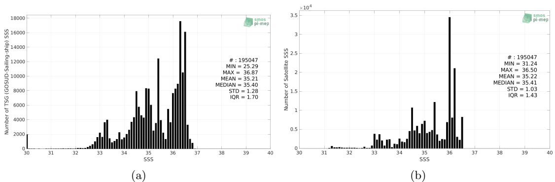
Figure 2: Histograms of SSS from TSG (GOSUD-Sailing-ship) (a) and SMOS SSS L4 v1 - Weekly (CMEMS-CNR) (b) considering all match-up pairs per bins of 0.1 over the Tropical Pacific Ocean Pi-MEP region and for the full satellite product period.
