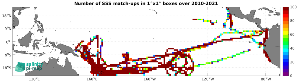
Figure 4: Number of SSS match-ups between TSG (GOSUD-Research-vessel) SSS and the SMOS SSS L4 v1 - Weekly (CMEMS-CNR) SSS product for the Tropical Pacific Ocean Pi-MEP region over 1^\circ \times 1^\circ boxes and for the full satellite product period.
