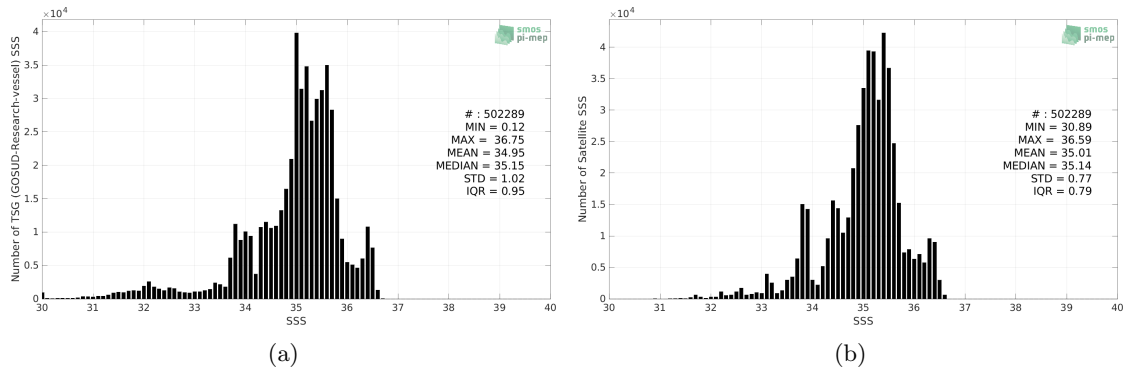
Figure 2: Histograms of SSS from TSG (GOSUD-Research-vessel) (a) and SMOS SSS L4 v1 - Weekly (CMEMS-CNR) (b) considering all match-up pairs per bins of 0.1 over the Tropical Pacific Ocean Pi-MEP region and for the full satellite product period.
