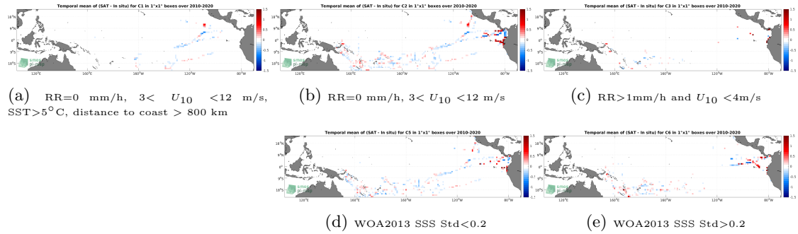
Figure 12: Temporal mean gridded over spatial boxes of size 1^{\circ}\times 1^{\circ} of \Delta SSS (SMOS SSS L4 v1 - Weekly (CMEMS-CNR) - TSG (GOSUD-Research-vessel)) for 5 different subdatasets corresponding to:RR=0 mm/h, 3 < U_{10} < 12 m/s, SST >5^{\circ}\text{C} , distance to coast > 800 km (a), RR=0 mm/h, 3 < U_{10} < 12 m/s (b), RR >1 mm/h and U_{10} < 4 m/s (c), WOA2013 SSS Std <0.2 (d), WOA2013 SSS Std >0.2 (e).
