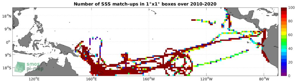
Figure 4: Number of SSS match-ups between TSG (GOSUD-Research-vessel) SSS and the SMOS SSS L4 v1 - Weekly (CMEMS-CNR) SSS product for the Tropical Pacific Ocean Pi-MEP region over 1^\circ \times 1^\circ boxes and for the full satellite product period.
