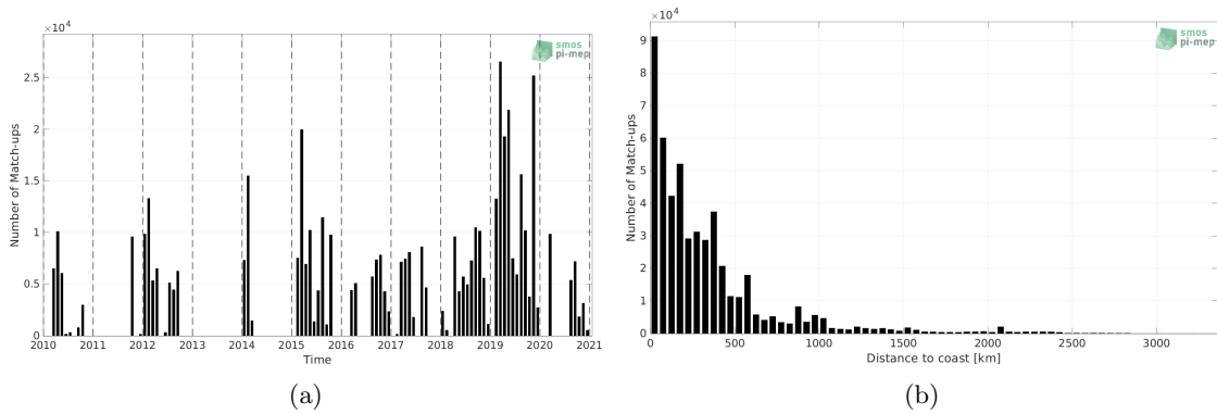
Figure 1: Number of match-ups between TSG (GOSUD-Research-vessel) and SMOS SSS L4 v1 - Weekly (CMEMS-CNR) SSS as a function of time (a) and as function of the distance to coast (b) over the Tropical Pacific Ocean Pi-MEP region and for the full satellite product period.
