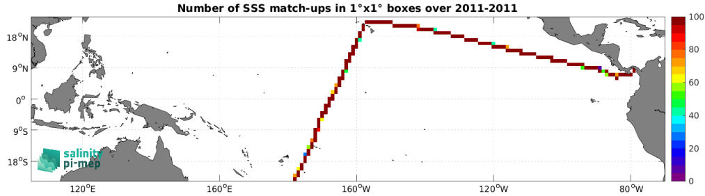
Figure 4: Number of SSS match-ups between TSG (CSIC-UTM) SSS and the SMOS SSS L4 v1 - Weekly (CMEMS-CNR) SSS product for the Tropical Pacific Ocean Pi-MEP region over 1^\circ \times 1^\circ boxes and for the full satellite product period.
