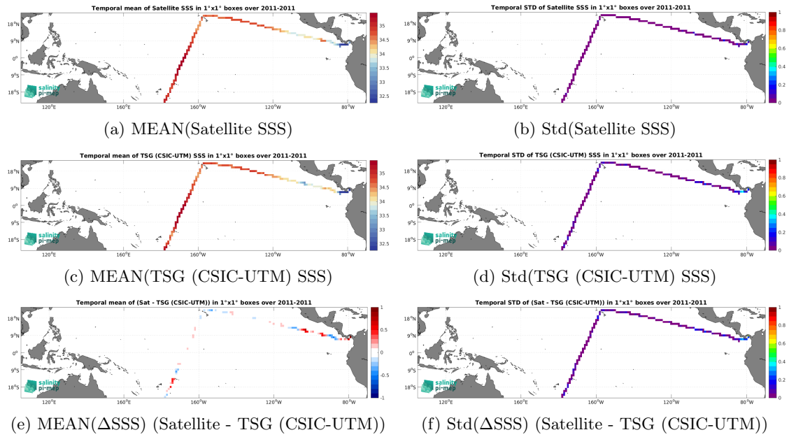
Figure 6: Temporal mean (left) and Std (right) of SSS from SMOS SSS L4 v1 - Weekly (CMEMS-CNR) (top), TSG (CSIC-UTM) (middle), and of \Delta SSS (Satellite - TSG (CSIC-UTM)). Only match-up pairs are used to generate these maps.
