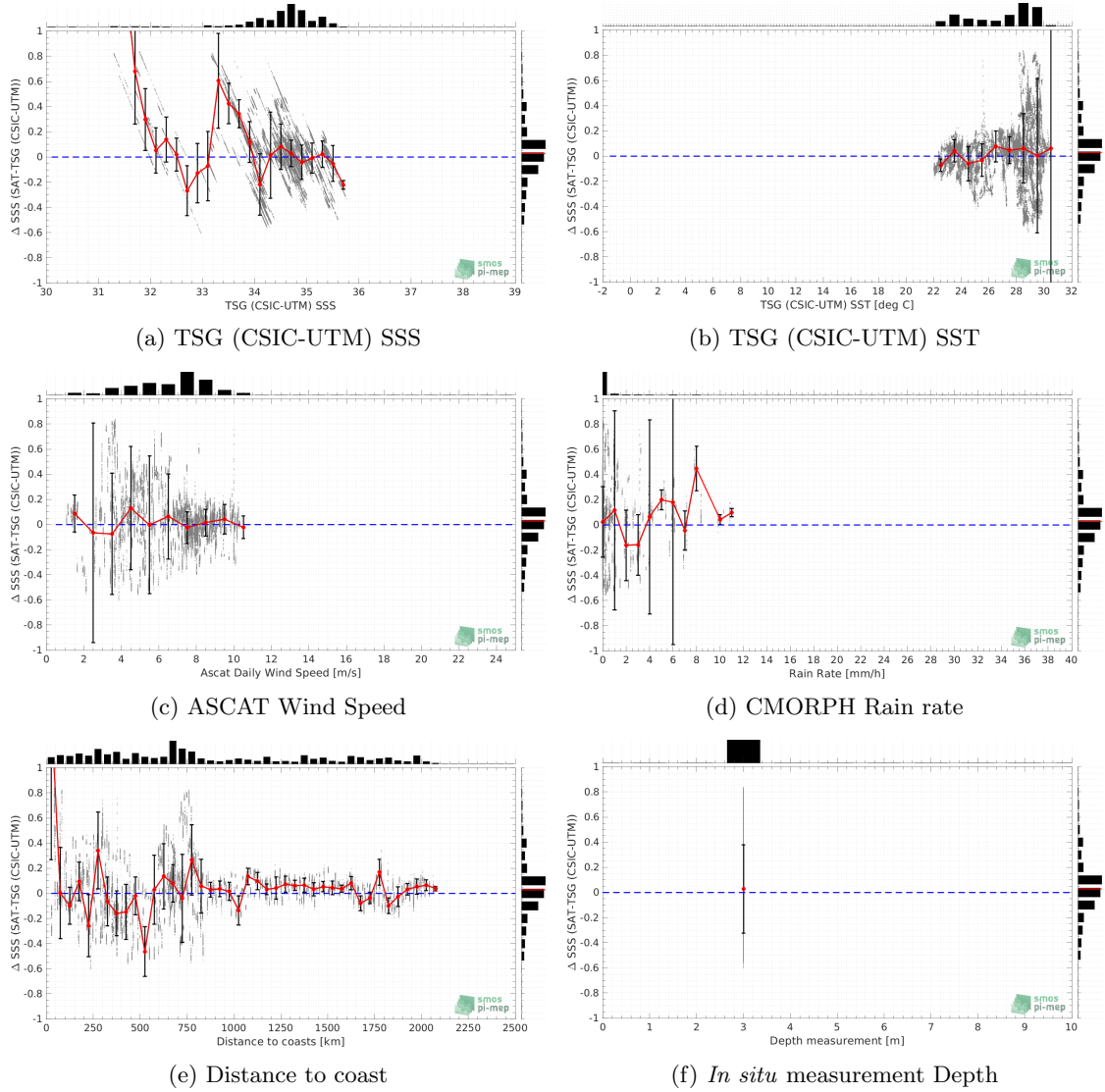
Figure 10: \Delta SSS (Satellite - TSG (CSIC-UTM)) sorted as function of TSG (CSIC-UTM) SSS values a), TSG (CSIC-UTM) SST b), ASCAT Wind speed c), CMORPH rain rate d), distance to coast (e) and in situ measurement depth (f). In all plots the median and Std of \Delta SSS for each bin is indicated by the red curves and black vertical thick bars ( \pm 1 Std)
