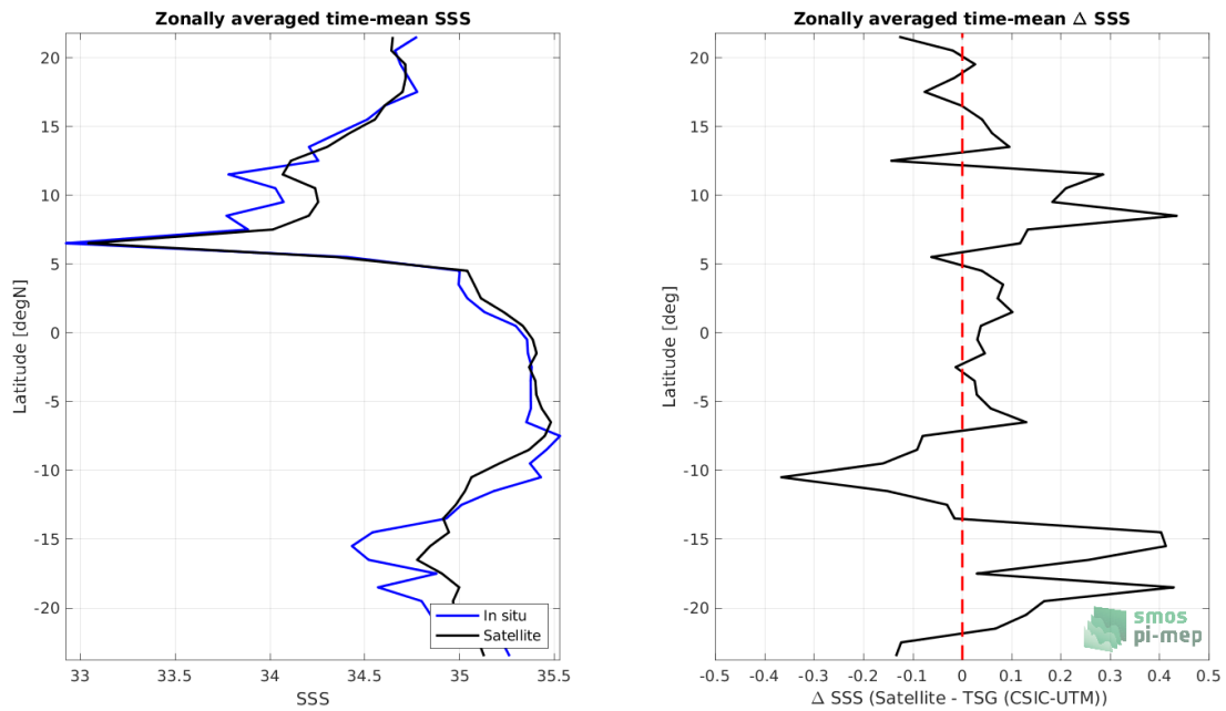
Figure 7: Left panel: Zonal mean SSS from SMOS SSS L4 v1 - Weekly (CMEMS-CNR) satellite product (black) and from TSG (CSIC-UTM) (blue). Right panel: Zonal mean of \Delta SSS (Satellite - TSG (CSIC-UTM)) for all the collected Pi-MEP match-up pairs estimated over the full satellite product period.
