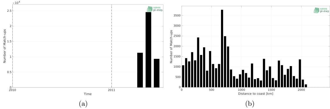
Figure 1: Number of match-ups between TSG (CSIC-UTM) and SMOS SSS L4 v1 - Weekly (CMEMS-CNR) SSS as a function of time (a) and as function of the distance to coast (b) over the Tropical Pacific Ocean Pi-MEP region and for the full satellite product period.
