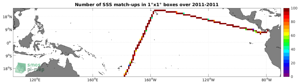
Figure 3: Number of SSS match-ups between TSG (CSIC-UTM) SSS and the SMOS SSS L4 v1 - Weekly (CMEMS-CNR) SSS product for the Tropical Pacific Ocean Pi-MEP region over 1^\circ \times 1^\circ boxes and for the full satellite product period.
