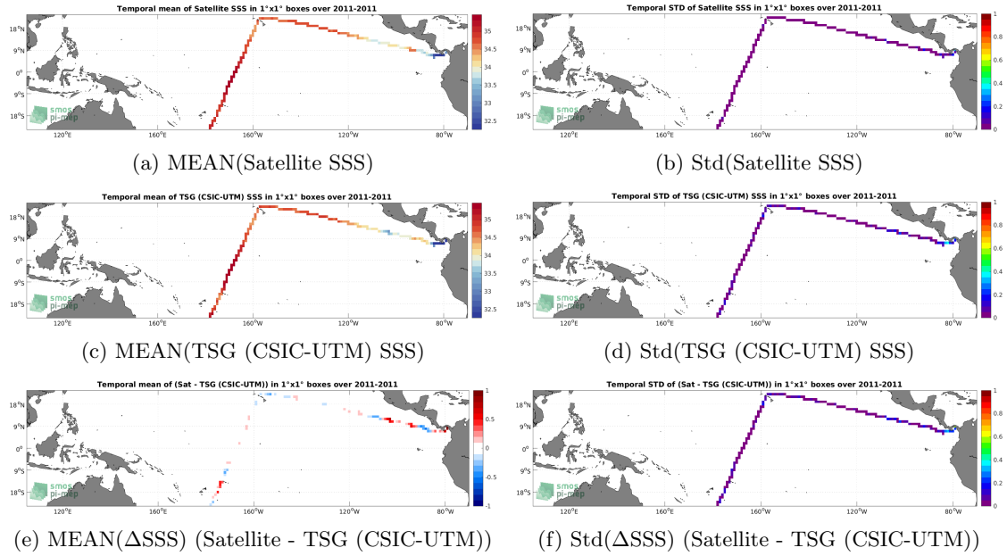
Figure 5: Temporal mean (left) and Std (right) of SSS from SMOS SSS L4 v1 - Weekly (CMEMS-CNR) (top), TSG (CSIC-UTM) (middle), and of \Delta SSS (Satellite - TSG (CSIC-UTM)). Only match-up pairs are used to generate these maps.
