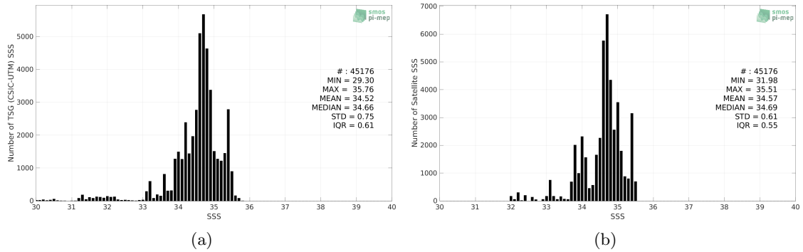
Figure 2: Histograms of SSS from TSG (CSIC-UTM) (a) and SMOS SSS L4 v1 - Weekly (CMEMS-CNR) (b) considering all match-up pairs per bins of 0.1 over the Tropical Pacific Ocean Pi-MEP region and for the full satellite product period.
