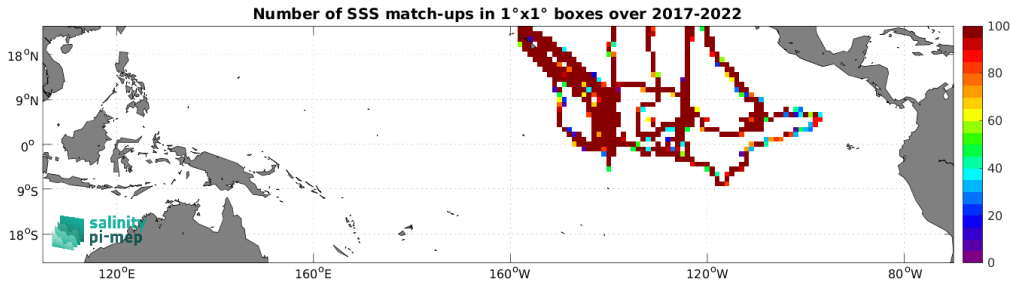
Figure 4: Number of SSS match-ups between Sailability SSS and the SMOS SSS L4 v1 - Weekly (CMEMS-CNR) SSS product for the Tropical Pacific Ocean Pi-MEP region over 1^\circ \times 1^\circ boxes and for the full satellite product period.
