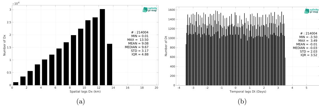
Figure 5: Histograms of the spatial (a) and temporal (b) lags between the location/time of the Sailability measurement and the date of the corresponding SMOS SSS L4 v1 - Weekly (CMEMS-CNR) SSS pixel.
