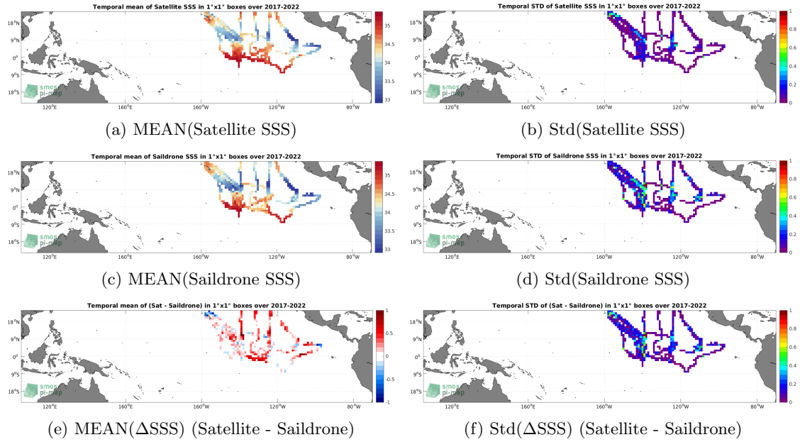
Figure 6: Temporal mean (left) and Std (right) of SSS from SMOS SSS L4 v1 - Weekly (CMEMS-CNR) (top), Saildrone (middle), and of \Delta SSS (Satellite - Saildrone). Only match-up pairs are used to generate these maps.
