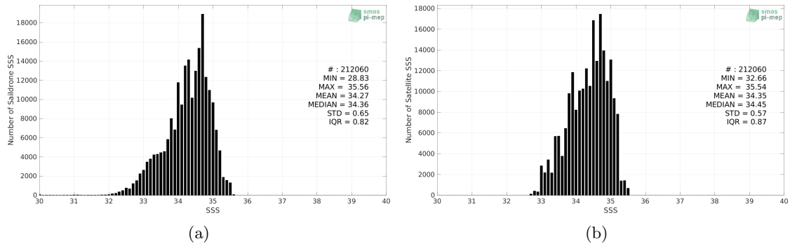
Figure 2: Histograms of SSS from Saildrone (a) and SMOS SSS L4 v1 - Weekly (CMEMS-CNR) (b) considering all match-up pairs per bins of 0.1 over the Tropical Pacific Ocean Pi-MEP region and for the full satellite product period.
