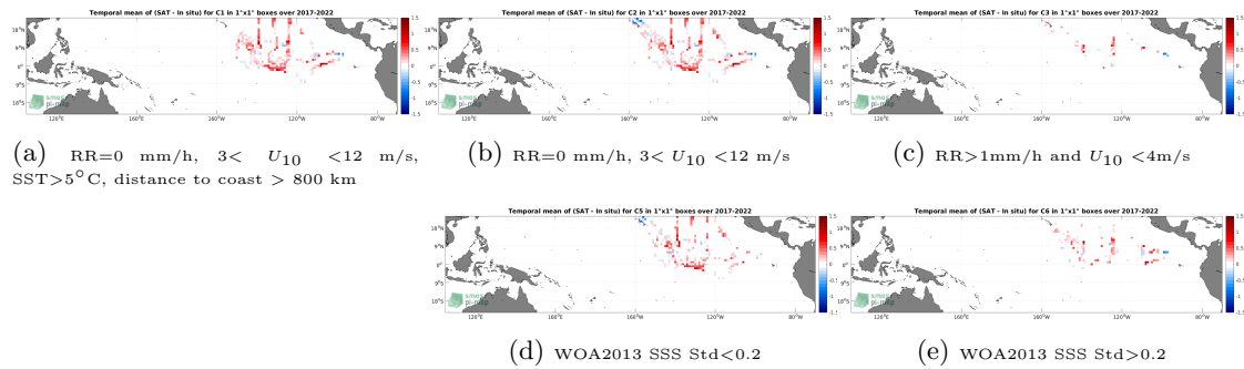
Figure 12: Temporal mean gridded over spatial boxes of size 1^\circ \times 1^\circ of \Delta SSS (SMOS SSS L4 v1 - Weekly (CMEMS-CNR) - Saildrone) for 5 different subdatasets corresponding to: RR=0 mm/h, 3 < U_{10} < 12 m/s, SST>5°C, distance to coast > 800 km (a), RR=0 mm/h, 3 < U_{10} < 12 m/s (b), RR>1mm/h and U_{10} < 4 m/s (c), WOA2013 SSS Std<0.2 (d), WOA2013 SSS Std>0.2 (e).
