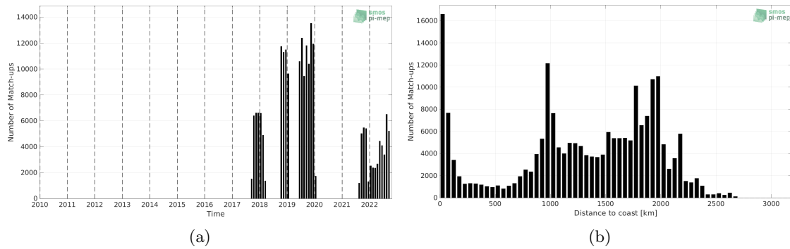
Figure 1: Number of match-ups between Saildrone and SMOS SSS L4 v1 - Weekly (CMEMS-CNR) SSS as a function of time (a) and as function of the distance to coast (b) over the Tropical Pacific Ocean Pi-MEP region and for the full satellite product period.
