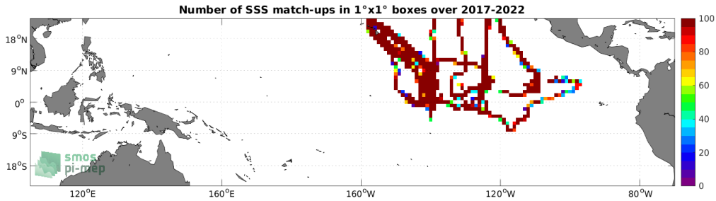
Figure 4: Number of SSS match-ups between Sairdrone SSS and the SMOS SSS L4 v1 - Weekly (CMEMS-CNR) SSS product for the Tropical Pacific Ocean Pi-MEP region over 1^\circ \times 1^\circ boxes and for the full satellite product period.
