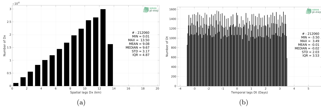
Figure 5: Histograms of the spatial (a) and temporal (b) lags between the location/time of the Sairdrone measurement and the date of the corresponding SMOS SSS L4 v1 - Weekly (CMEMS-CNR) SSS pixel.
