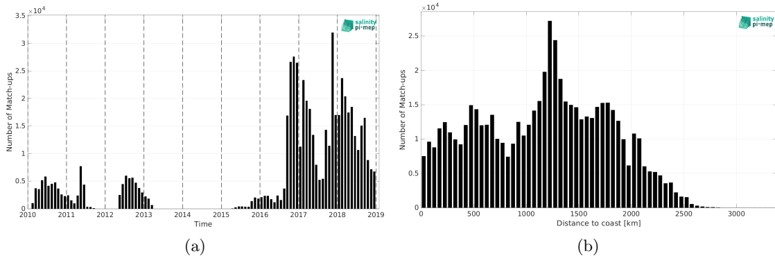
Figure 1: Number of match-ups between Surface drifters and SMOS SSS L4 v1 - Weekly (CMEMS-CNR) SSS as a function of time (a) and as function of the distance to coast (b) over the Tropical Pacific Ocean Pi-MEP region and for the full satellite product period.
