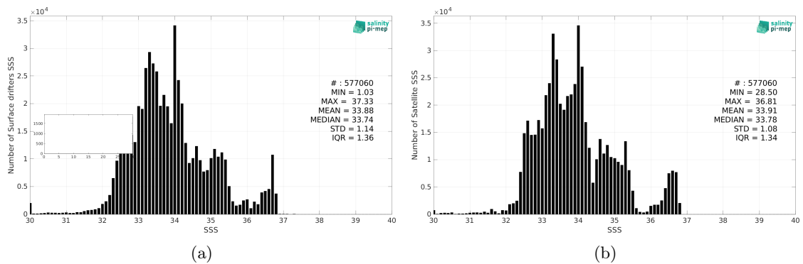
Figure 2: Histograms of SSS from Surface drifters (a) and SMOS SSS L4 v1 - Weekly (CMEMS-CNR) (b) considering all match-up pairs per bins of 0.1 over the Tropical Pacific Ocean Pi-MEP region and for the full satellite product period.
