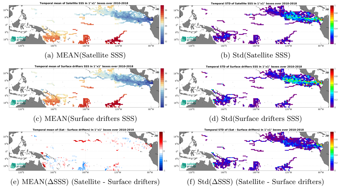
Figure 5: Temporal mean (left) and Std (right) of SSS from SMOS SSS L4 v1 - Weekly (CMEMS-CNR) (top), Surface drifters (middle), and of \Delta SSS (Satellite - Surface drifters). Only match-up pairs are used to generate these maps.
