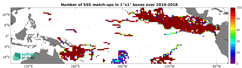
Figure 3: Number of SSS match-ups between Surface drifters SSS and the SMOS SSS L4 v1 - Weekly (CMEMS-CNR) SSS product for the Tropical Pacific Ocean Pi-MEP region over 1^\circ \times 1^\circ boxes and for the full satellite product period.
