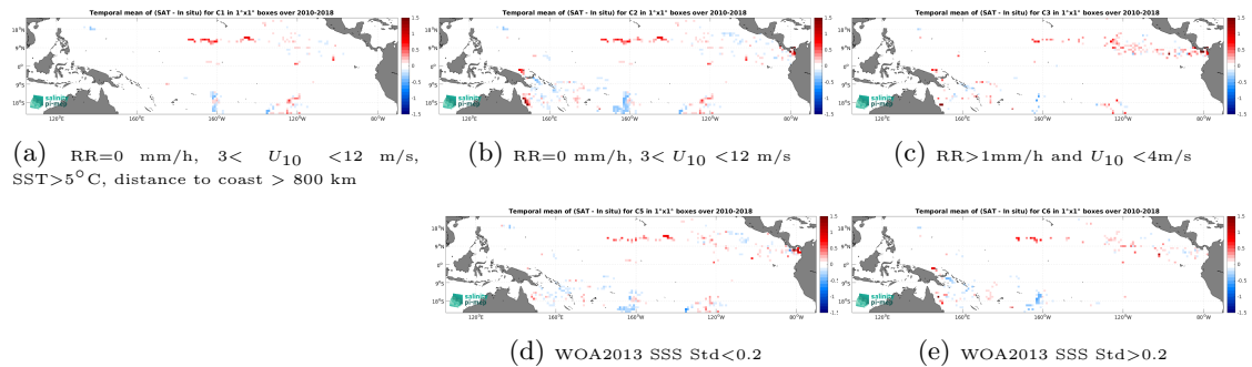
Figure 11: Temporal mean gridded over spatial boxes of size 1^\circ \times 1^\circ of \Delta SSS (SMOS SSS L4 v1 - Weekly (CMEMS-CNR) - Surface drifters) for 5 different subdatasets corresponding to:RR=0 mm/h, 3 < U_{10} < 12 m/s, SST > 5^\circ\text{C} , distance to coast > 800 km (a), RR=0 mm/h, 3 < U_{10} < 12 m/s (b), RR > 1 mm/h and U_{10} < 4 m/s (c), WOA2013 SSS Std < 0.2 (d), WOA2013 SSS Std > 0.2 (e).
