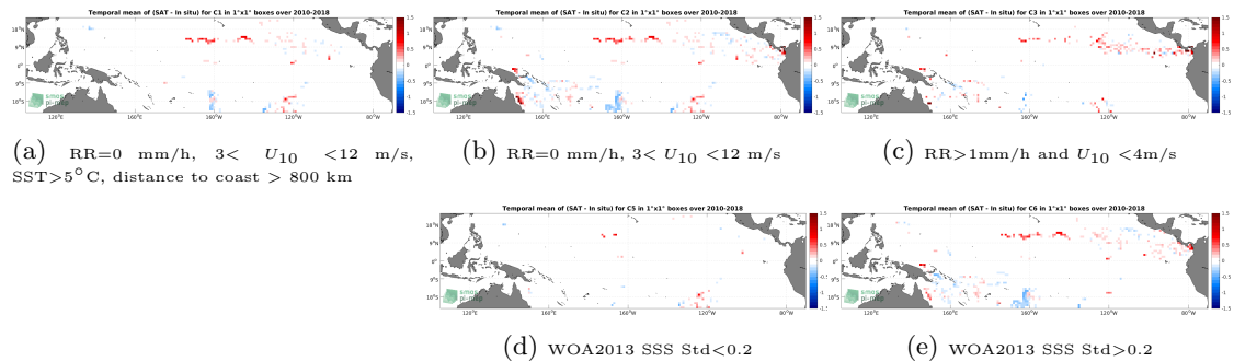
Figure 11: Temporal mean gridded over spatial boxes of size 1^\circ \times 1^\circ of \Delta SSS (SMOS SSS L4 v1 - Weekly (CMEMS-CNR) - Surface drifters) for 5 different subdatasets corresponding to:RR=0 mm/h, 3 < U_{10} < 12 m/s, SST > 5^\circ\text{C} , distance to coast > 800 km (a), RR=0 mm/h, 3 < U_{10} < 12 m/s (b), RR > 1 mm/h and U_{10} < 4 m/s (c), WOA2013 SSS Std < 0.2 (d), WOA2013 SSS Std > 0.2 (e).
