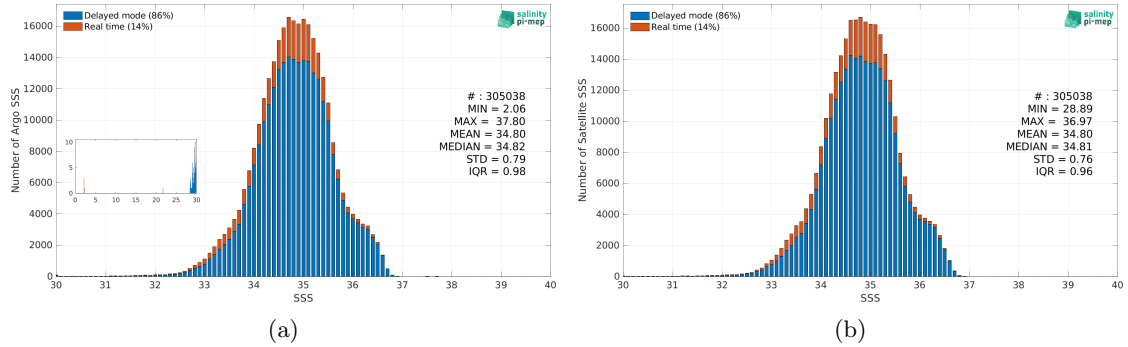
Figure 2: Histograms of SSS from Argo (a) and SMOS SSS L4 v1 - Weekly (CMEMS-CNR) (b) considering all match-up pairs per bins of 0.1 over the Tropical Pacific Ocean Pi-MEP region and for the full satellite product period.
