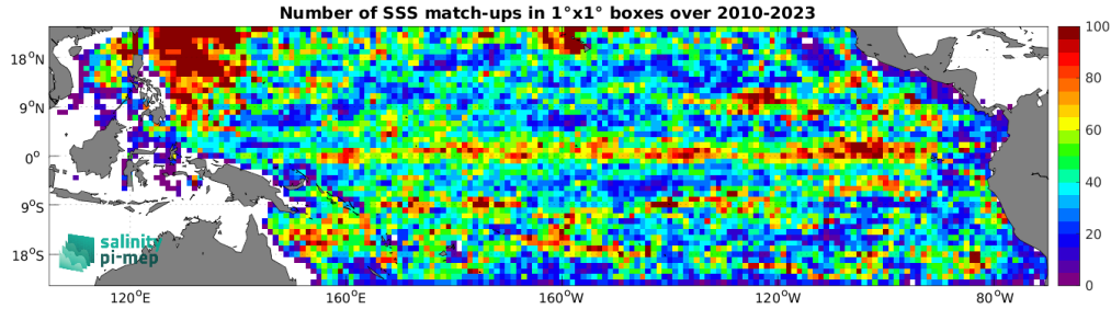
Figure 4: Number of SSS match-ups between Argo SSS and the SMOS SSS L4 v1 - Weekly (CMEMS-CNR) SSS product for the Tropical Pacific Ocean Pi-MEP region over 1^\circ \times 1^\circ boxes and for the full satellite product period.
