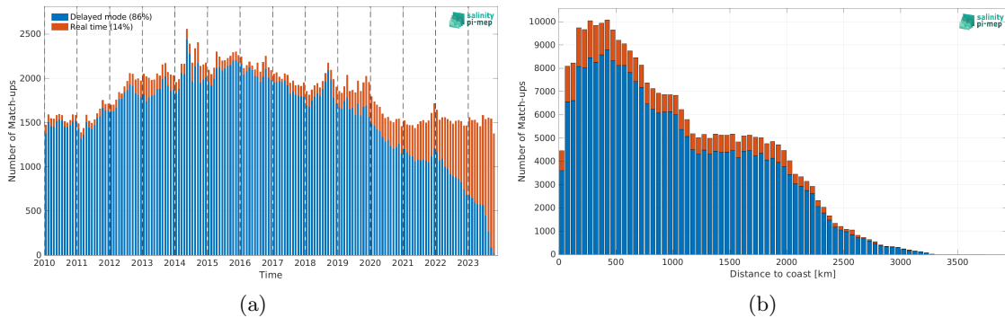
Figure 1: Number of match-ups between Argo and SMOS SSS L4 v1 - Weekly (CMEMS-CNR) SSS as a function of time (a) and as function of the distance to coast (b) over the Tropical Pacific Ocean Pi-MEP region and for the full satellite product period.
