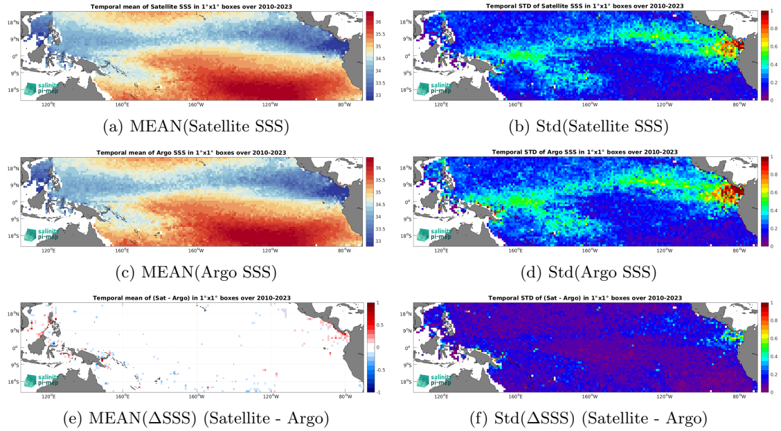
Figure 6: Temporal mean (left) and Std (right) of SSS from SMOS SSS L4 v1 - Weekly (CMEMS-CNR) (top), Argo (middle), and of \Delta SSS (Satellite - Argo). Only match-up pairs are used to generate these maps.
