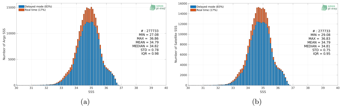
Figure 2: Histograms of SSS from Argo (a) and SMOS SSS L4 v1 - Weekly (CMEMS-CNR) (b) considering all match-up pairs per bins of 0.1 over the Tropical Pacific Ocean Pi-MEP region and for the full satellite product period.
