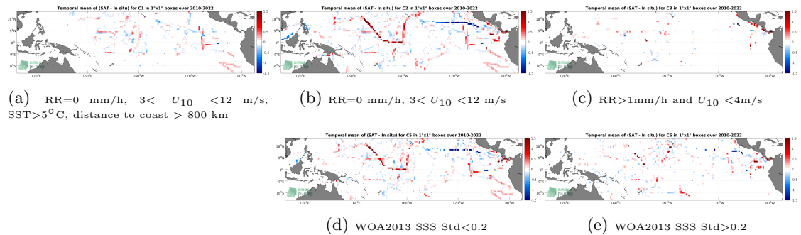
Figure 12: Temporal mean gridded over spatial boxes of size 1^\circ \times 1^\circ of \Delta SSS (SMOS SSS L4 v1 - Monthly (CMEMS-CNR) - TSG (SAMOS)) for 5 different subdatasets corresponding to: RR=0 mm/h, 3 < U_{10} < 12 m/s, SST > 5^\circ\text{C} , distance to coast > 800 km (a), RR=0 mm/h, 3 < U_{10} < 12 m/s (b), RR > 1 mm/h and U_{10} < 4 m/s (c), WOA2013 SSS Std < 0.2 (d), WOA2013 SSS Std > 0.2 (e).
