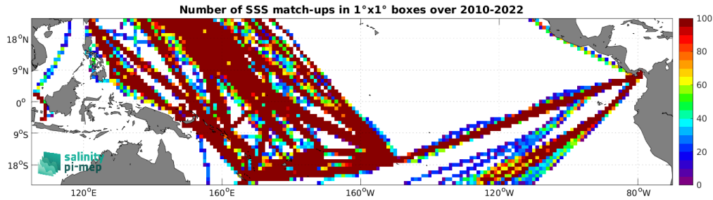
Figure 5: Number of SSS match-ups between TSG (LEGOS-DM) SSS and the SMOS SSS L4 v1 - Monthly (CMEMS-CNR) SSS product for the Tropical Pacific Ocean Pi-MEP region over 1^\circ \times 1^\circ boxes and for the full satellite product period.
