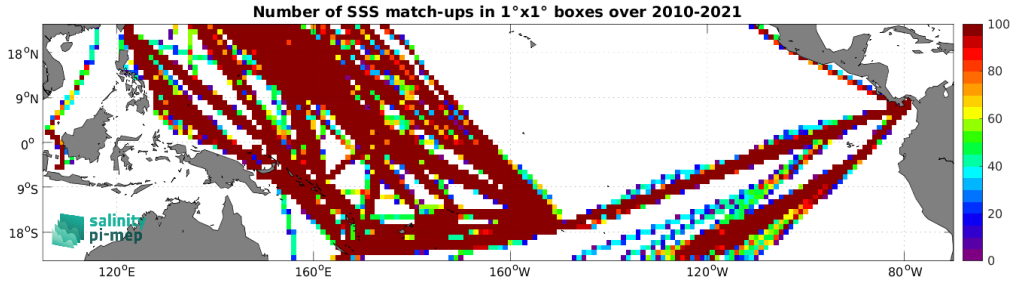
Figure 4: Number of SSS match-ups between TSG (LEGOS-DM) SSS and the SMOS SSS L4 v1 - Monthly (CMEMS-CNR) SSS product for the Tropical Pacific Ocean Pi-MEP region over 1^\circ \times 1^\circ boxes and for the full satellite product period.
