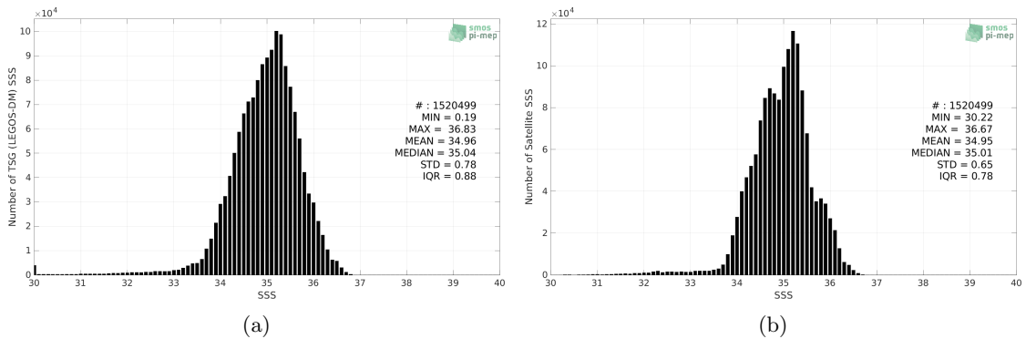
Figure 2: Histograms of SSS from TSG (LEGOS-DM) (a) and SMOS SSS L4 v1 - Monthly (CMEMS-CNR) (b) considering all match-up pairs per bins of 0.1 over the Tropical Pacific Ocean Pi-MEP region and for the full satellite product period.
