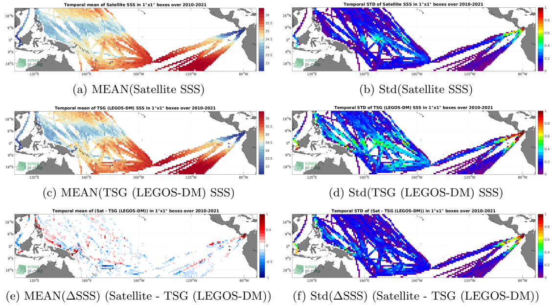
Figure 6: Temporal mean (left) and Std (right) of SSS from SMOS SSS L4 v1 - Monthly (CMEMS-CNR) (top), TSG (LEGOS-DM) (middle), and of \Delta SSS (Satellite - TSG (LEGOS-DM)). Only match-up pairs are used to generate these maps.
