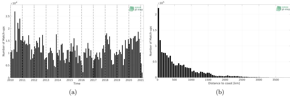
Figure 1: Number of match-ups between TSG (LEGOS-DM) and SMOS SSS L4 v1 - Monthly (CMEMS-CNR) SSS as a function of time (a) and as function of the distance to coast (b) over the Tropical Pacific Ocean Pi-MEP region and for the full satellite product period.
