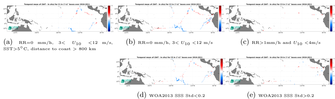
Figure 14: Temporal mean gridded over spatial boxes of size 1^\circ \times 1^\circ of \Delta SSS (SMOS SSS L4 v1 - Monthly (CMEMS-CNR) - TSG (GOSUD-Sailing-ship)) for 5 different subdatasets corresponding to:RR=0 mm/h, 3 < U_{10} < 12 m/s, SST > 5^\circ C, distance to coast > 800 km (a), RR=0 mm/h, 3 < U_{10} < 12 m/s (b), RR > 1 mm/h and U_{10} < 4 m/s (c), WOA2013 SSS Std < 0.2 (d), WOA2013 SSS Std > 0.2 (e).
