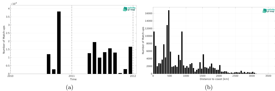
Figure 2: Number of match-ups between TSG (GOSUD-Sailing-ship) and SMOS SSS L4 v1 - Monthly (CMEMS-CNR) SSS as a function of time (a) and as function of the distance to coast (b) over the Tropical Pacific Ocean Pi-MEP region and for the full satellite product period.
