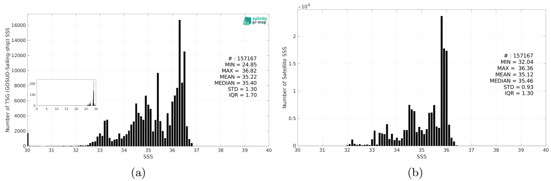
Figure 3: Histograms of SSS from TSG (GOSUD-Sailing-ship) (a) and SMOS SSS L4 v1 - Monthly (CMEMS-CNR) (b) considering all match-up pairs per bins of 0.1 over the Tropical Pacific Ocean Pi-MEP region and for the full satellite product period.
