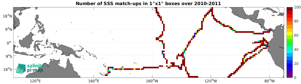
Figure 5: Number of SSS match-ups between TSG (GOSUD-Sailing-ship) SSS and the SMOS SSS L4 v1 - Monthly (CMEMS-CNR) SSS product for the Tropical Pacific Ocean Pi-MEP region over 1^\circ \times 1^\circ boxes and for the full satellite product period.
