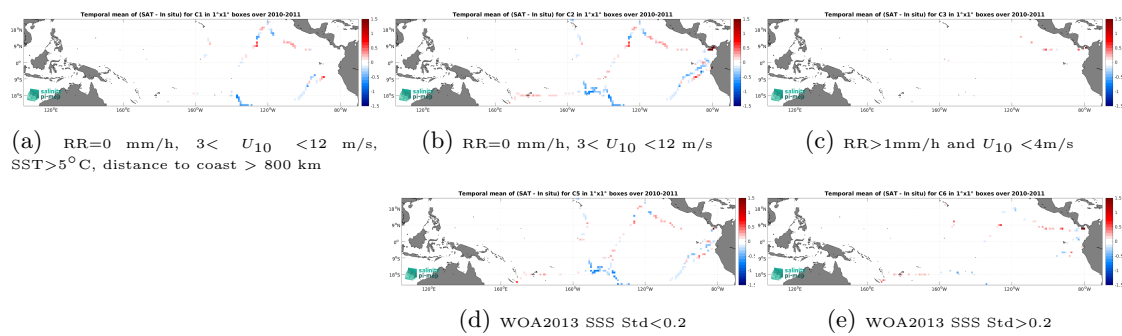
Figure 12: Temporal mean gridded over spatial boxes of size 1^\circ \times 1^\circ of \Delta\text{SSS} (SMOS SSS L4 v1 - Monthly (CMEMS-CNR) - TSG (GOSUD-Sailing-ship)) for 5 different subdatasets corresponding to: RR=0 mm/h, 3 < U_{10} < 12 m/s, SST > 5^\circ\text{C} , distance to coast > 800 km (a), RR=0 mm/h, 3 < U_{10} < 12 m/s (b), RR > 1 mm/h and U_{10} < 4 m/s (c), WOA2013 SSS Std < 0.2 (d), WOA2013 SSS Std > 0.2 (e).
