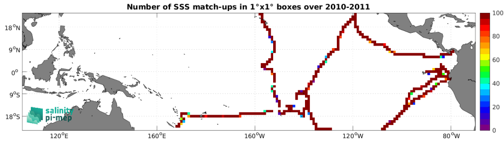
Figure 4: Number of SSS match-ups between TSG (GOSUD-Sailing-ship) SSS and the SMOS SSS L4 v1 - Monthly (CMEMS-CNR) SSS product for the Tropical Pacific Ocean Pi-MEP region over 1^\circ \times 1^\circ boxes and for the full satellite product period.
