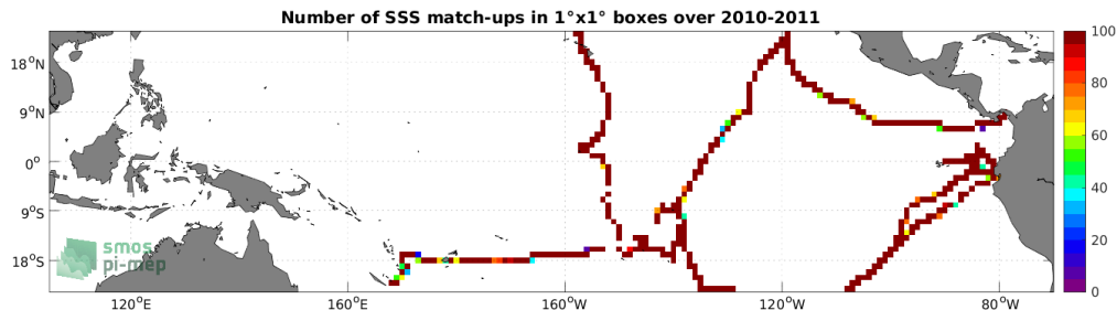
Figure 4: Number of SSS match-ups between TSG (GOSUD-Sailing-ship) SSS and the SMOS SSS L4 v1 - Monthly (CMEMS-CNR) SSS product for the Tropical Pacific Ocean Pi-MEP region over 1^\circ \times 1^\circ boxes and for the full satellite product period.
