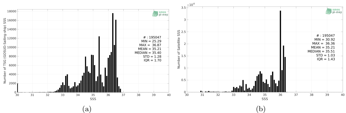
Figure 2: Histograms of SSS from TSG (GOSUD-Sailing-ship) (a) and SMOS SSS L4 v1 - Monthly (CMEMS-CNR) (b) considering all match-up pairs per bins of 0.1 over the Tropical Pacific Ocean Pi-MEP region and for the full satellite product period.
