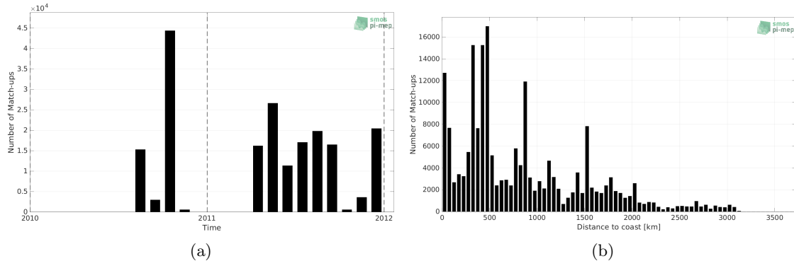
Figure 1: Number of match-ups between TSG (GOSUD-Sailing-ship) and SMOS SSS L4 v1 - Monthly (CMEMS-CNR) SSS as a function of time (a) and as function of the distance to coast (b) over the Tropical Pacific Ocean Pi-MEP region and for the full satellite product period.
