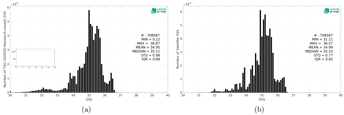
Figure 2: Histograms of SSS from TSG (GOSUD-Research-vessel) (a) and SMOS SSS L4 v1 - Monthly (CMEMS-CNR) (b) considering all match-up pairs per bins of 0.1 over the Tropical Pacific Ocean Pi-MEP region and for the full satellite product period.
