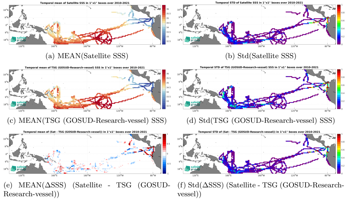
Figure 6: Temporal mean (left) and Std (right) of SSS from SMOS SSS L4 v1 - Monthly (CMEMS-CNR) (top), TSG (GOSUD-Research-vessel) (middle), and of \Delta SSS (Satellite - TSG (GOSUD-Research-vessel)). Only match-up pairs are used to generate these maps.
