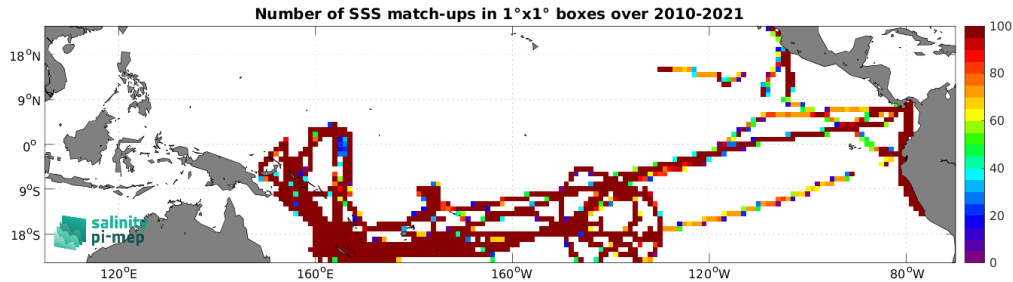
Figure 4: Number of SSS match-ups between TSG (GOSUD-Research-vessel) SSS and the SMOS SSS L4 v1 - Monthly (CMEMS-CNR) SSS product for the Tropical Pacific Ocean Pi-MEP region over 1^\circ \times 1^\circ boxes and for the full satellite product period.
