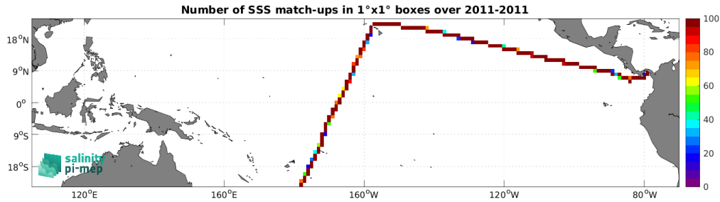
Figure 5: Number of SSS match-ups between TSG (CSIC-UTM) SSS and the SMOS SSS L4 v1 - Monthly (CMEMS-CNR) SSS product for the Tropical Pacific Ocean Pi-MEP region over 1^\circ \times 1^\circ boxes and for the full satellite product period.
