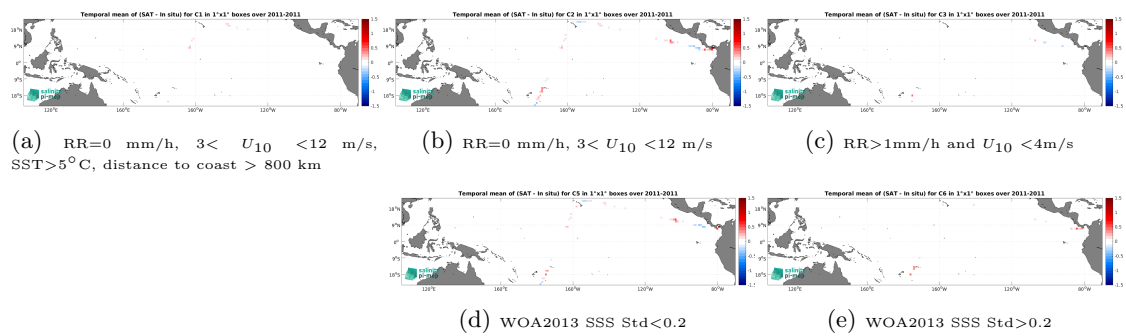
Figure 14: Temporal mean gridded over spatial boxes of size 1^\circ \times 1^\circ of \Delta SSS (SMOS SSS L4 v1 - Monthly (CMEMS-CNR) - TSG (CSIC-UTM)) for 5 different subdatasets corresponding to:RR=0 mm/h, 3 < U_{10} < 12 m/s, SST >5^\circ\text{C} , distance to coast > 800 km (a), RR=0 mm/h, 3 < U_{10} < 12 m/s (b), RR >1 mm/h and U_{10} < 4 m/s (c), WOA2013 SSS Std <0.2 (d), WOA2013 SSS Std >0.2 (e).
