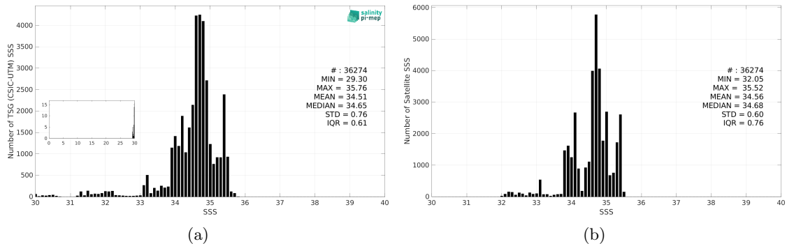
Figure 3: Histograms of SSS from TSG (CSIC-UTM) (a) and SMOS SSS L4 v1 - Monthly (CMEMS-CNR) (b) considering all match-up pairs per bins of 0.1 over the Tropical Pacific Ocean Pi-MEP region and for the full satellite product period.
