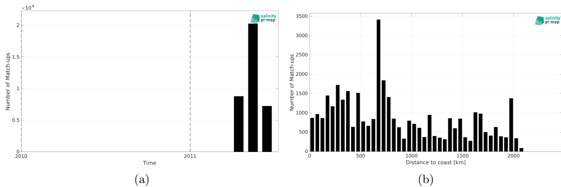
Figure 2: Number of match-ups between TSG (CSIC-UTM) and SMOS SSS L4 v1 - Monthly (CMEMS-CNR) SSS as a function of time (a) and as function of the distance to coast (b) over the Tropical Pacific Ocean Pi-MEP region and for the full satellite product period.
