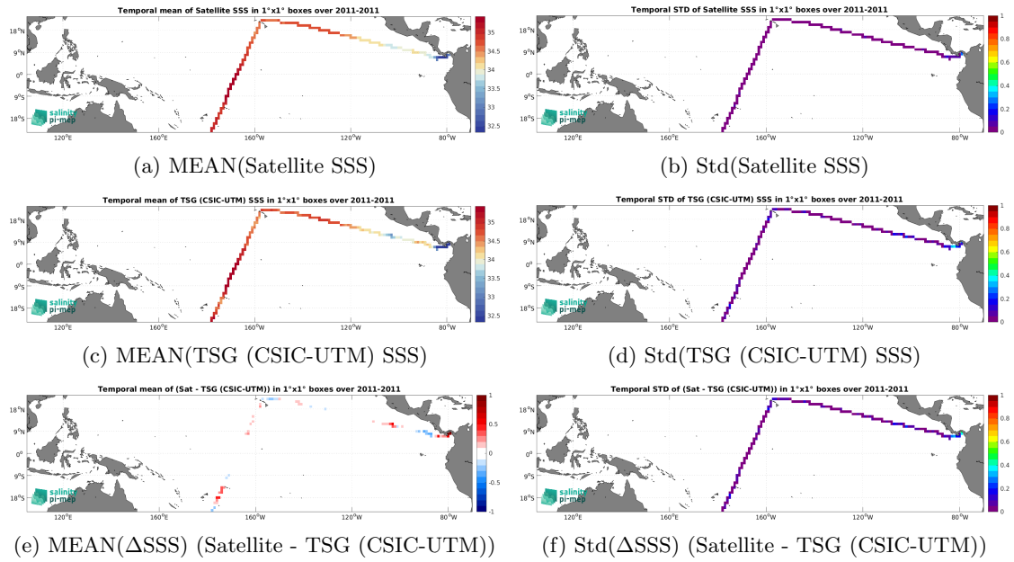
Figure 7: Temporal mean (left) and Std (right) of SSS from SMOS SSS L4 v1 - Monthly (CMEMS-CNR) (top), TSG (CSIC-UTM) (middle), and of \Delta SSS (Satellite - TSG (CSIC-UTM)). Only match-up pairs are used to generate these maps.
