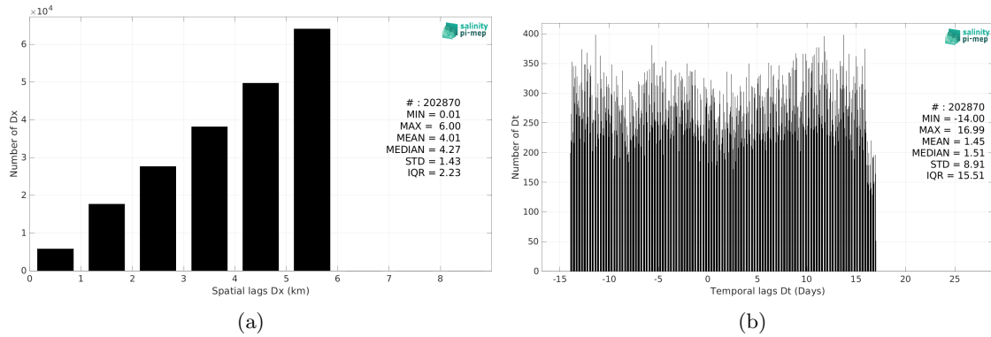
Figure 6: Histograms of the spatial (a) and temporal (b) lags between the location/time of the Sairdrone measurement and the date of the corresponding SMOS SSS L4 v1 - Monthly (CMEMS-CNR) SSS pixel.
